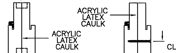
COMBINATION WOOD MULLION (BOXED)
