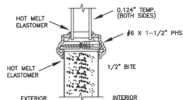
TYPICAL GLAZING DETAIL NON-IMPACT GLASS
