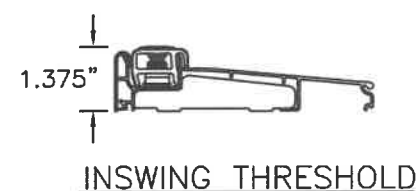
DETAIL "D"
