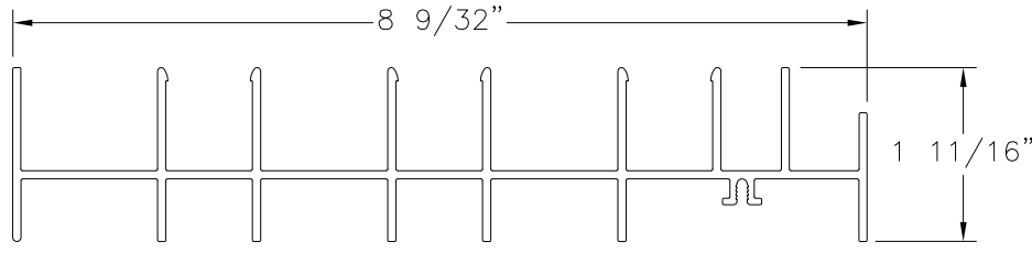
FRAME JAMB 3TRACK, FINLESS ALUMINUM 6005-T5 (M-2528)
