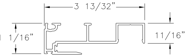
POCKET HOOK STRIP WITHOUT OPTIONAL RISER ALUMINUM 6063-T5 (M-2533)
