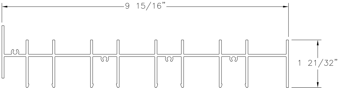
FRAME HEAD 4TRACK, FLANGE ALUMINUM 6005-T5 (M-2526)
