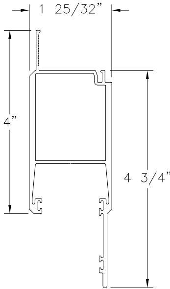
PANEL TOP STILE, OUTSIDE CORNER ALUMINUM 6005-T5 (M-2514)
