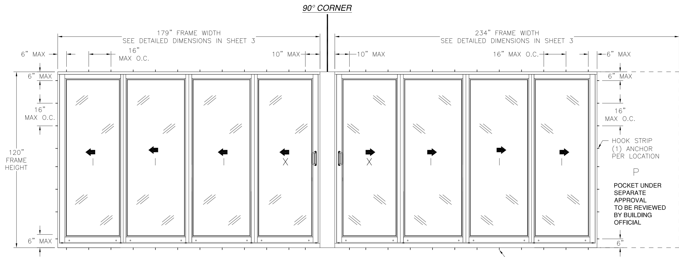
SERIES 120/130/140 ALUMINUM SGD OUTSIDE CORNER NON-IMPACT EXTERIOR VIEW
