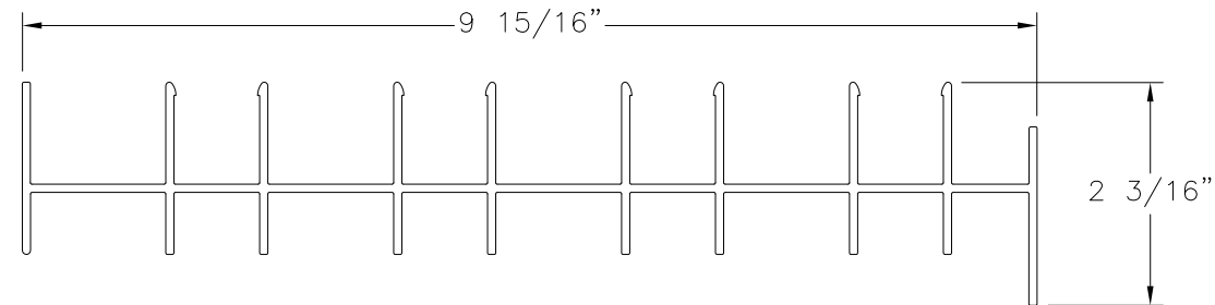
FRAME JAMB 4TRACK, FLANGE ALUMINUM 6005-T5 (M-2529)
