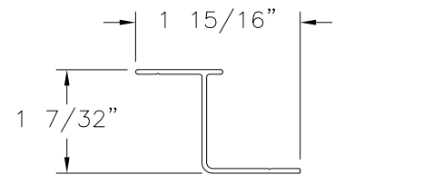
FIXED PANEL STILE RETAINER ALUMINUM 6063-T5 (M-2519)
