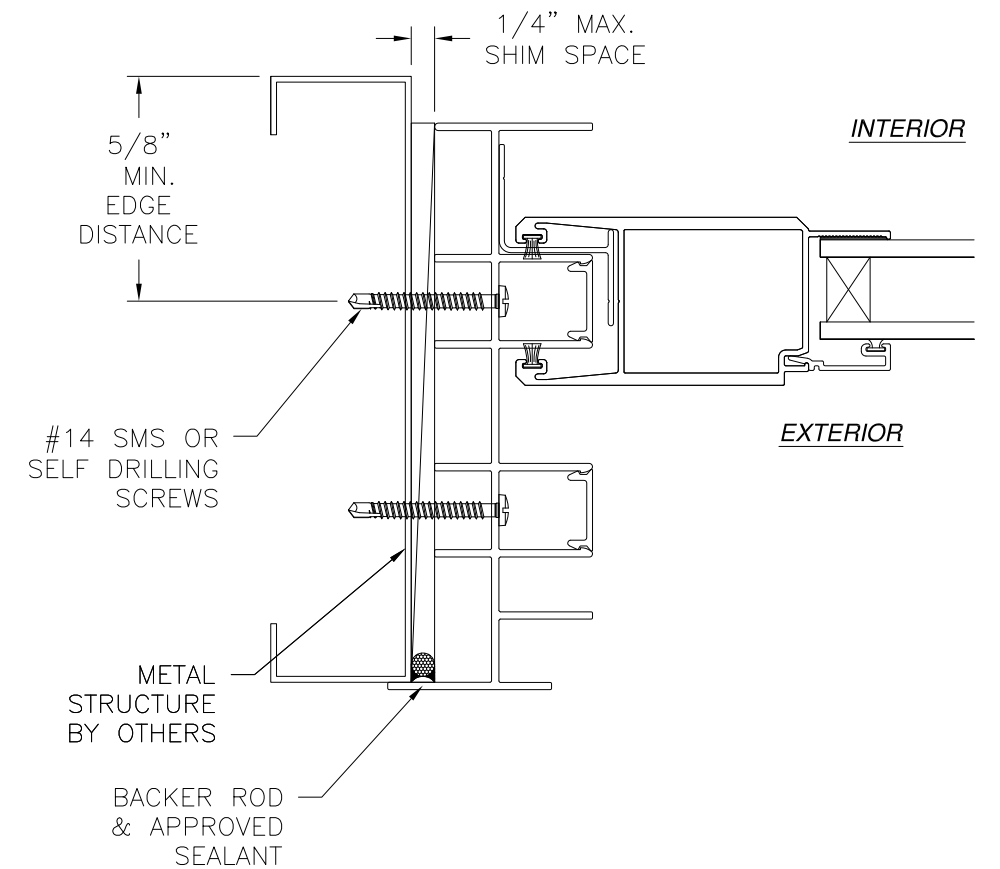
JAMB INSTALLATION DETAIL METAL STRUCTURE INSTALLATION
