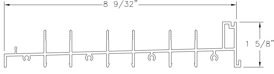
FRAME SILL 3TRACK ALUMINUM 6005-T5 (M-2527)
