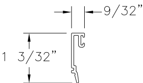
GLAZING BEAD ALUMINUM 6063-T5 (M-2505)
