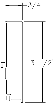
3 1/2" SILL EXTENDER ALUMINUM 6063-T5 .062" THICK (M-2531)
