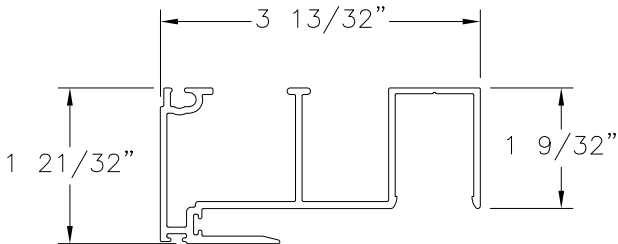
POCKET HOOK STRIP WITH OPTIONAL RISER ALUMINUM 6063-T5 (M-2534)
