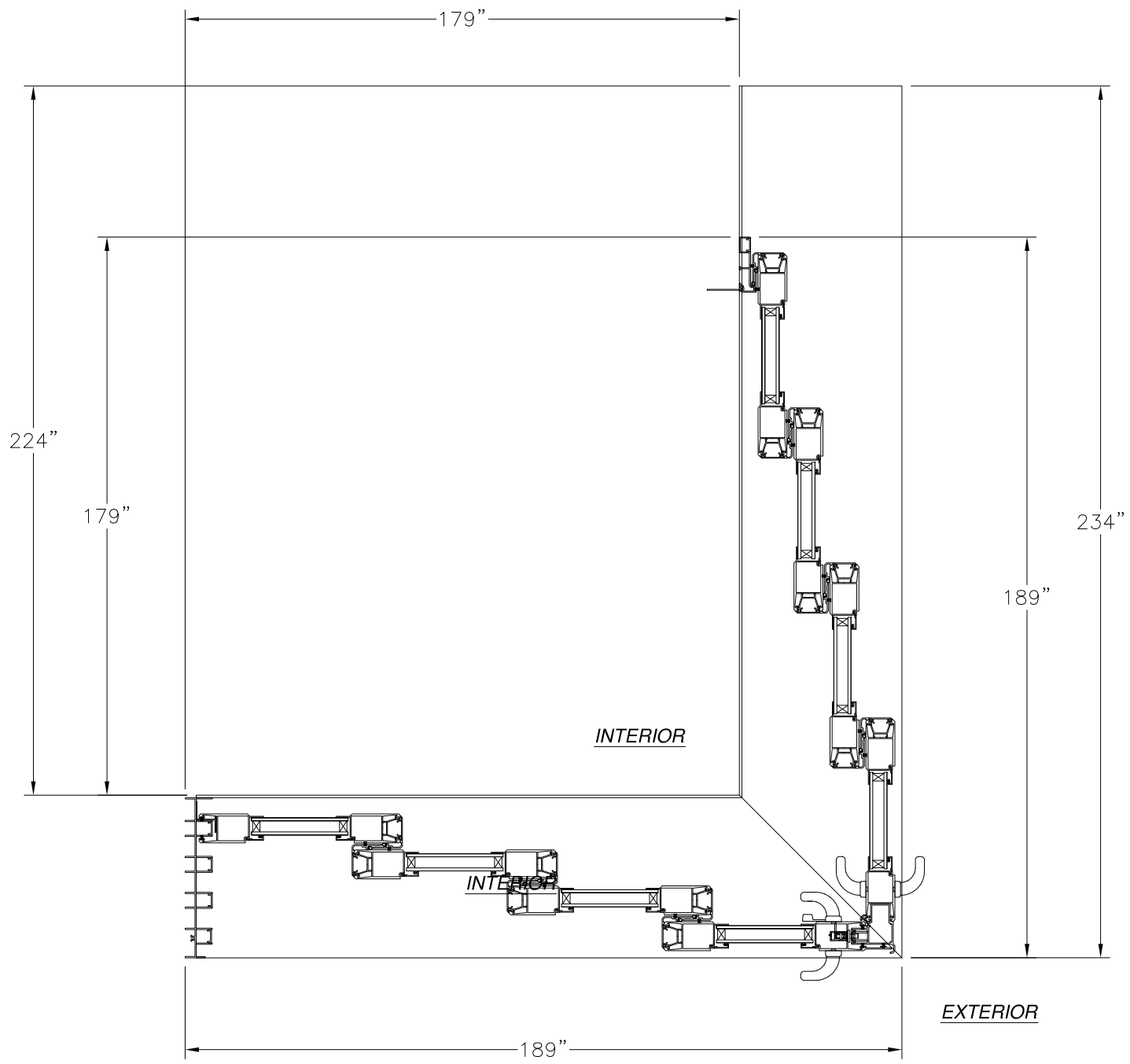
SERIES 120/130/140 ALUMINUM SGD OUTSIDE CORNER PLAN VIEW
