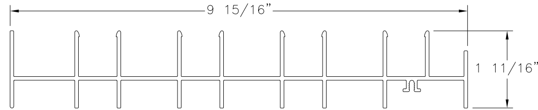
FRAME JAMB 4TRACK, FINLESS ALUMINUM 6005-T5 (M-2528)
