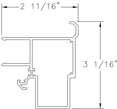
CORNER PANEL ADAPTER ALUMINUM 6005-T5 (M-2515)
