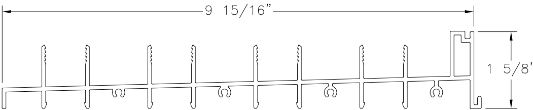
FRAME SILL 4TRACK ALUMINUM 6005-T5 (M-2527)
