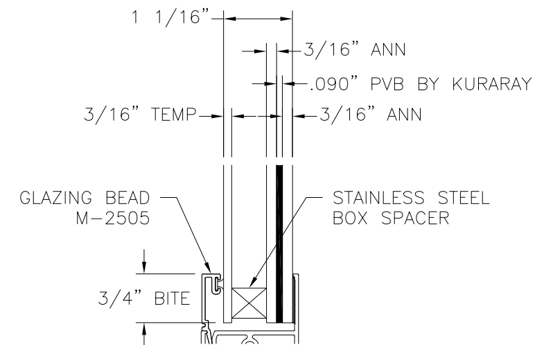
GLAZING DETAIL B
