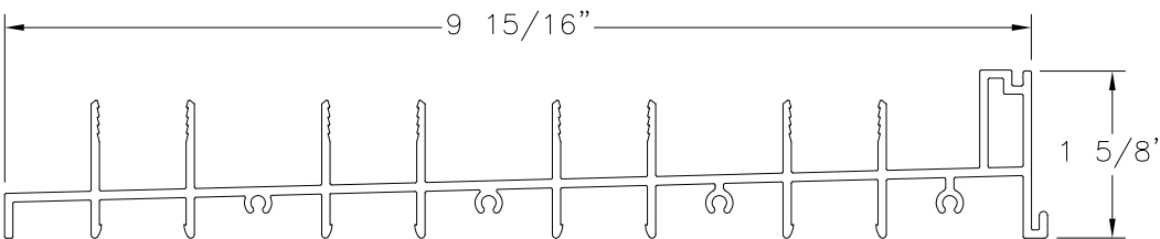
FRAME SILL 4TRACK ALUMINUM 6005-T5 (M-2522)
