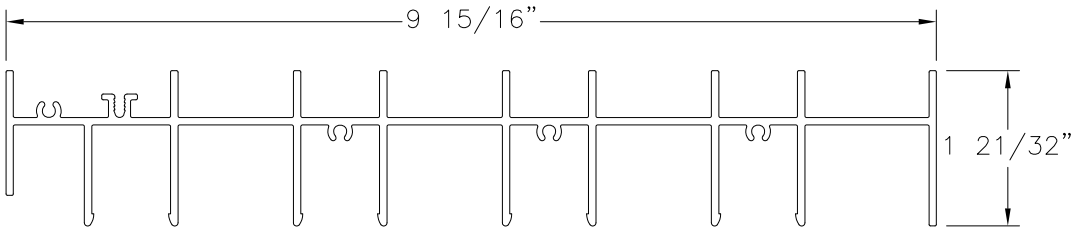
FRAME HEAD 4TRACK, FINLESS ALUMINUM 6005-T5 (M-2520)
