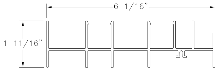
FRAME JAMB 2TRACK, FINLESS ALUMINUM 6005-T5 (M-2523)
