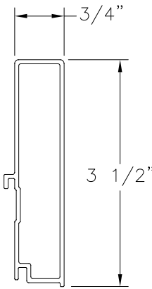
3 1/2" SILL EXTENDER ALUMINUM 6063-T5 .062" THICK
