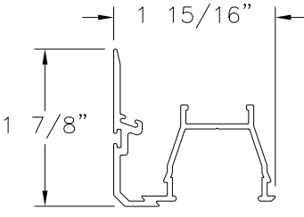
PANEL INTERLOCK ALUMINUM 6005-T5 (M-2503)
