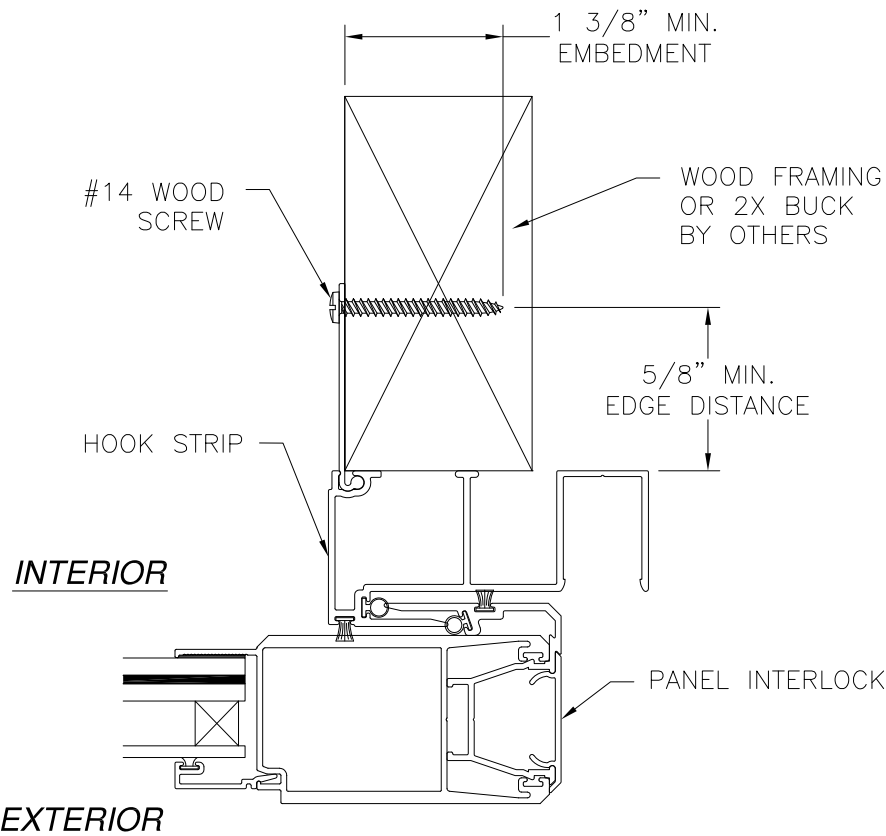
HOOK STRIP (M-2534) INSTALLATION 2X BUCK/WOOD FRAMING
