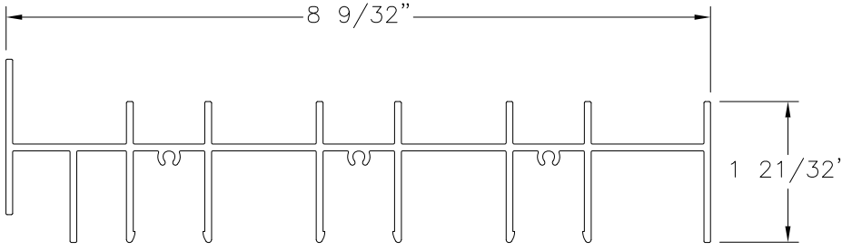
FRAME HEAD 3TRACK, FLANGE ALUMINUM 6005-T5 (M-2520)
