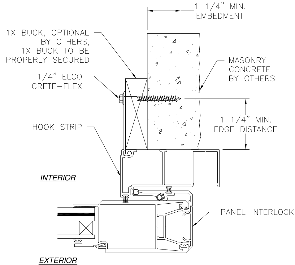
HOOK STRIP (M-2534) INSTALLATION MASONRY/CONCRETE
