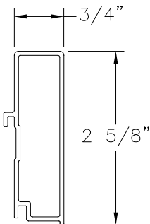
2 5/8" SILL EXTENDER ALUMINUM 6063-T5 .062" THICK
