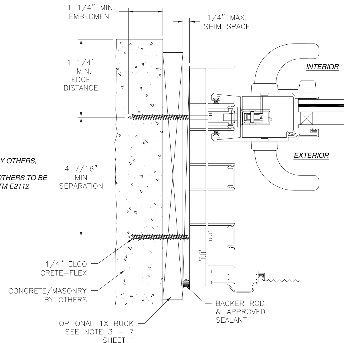
JAMB INSTALLATION DETAIL CONCRETE/MASONRY INSTALLATION SIGNED: 11/03/2022
