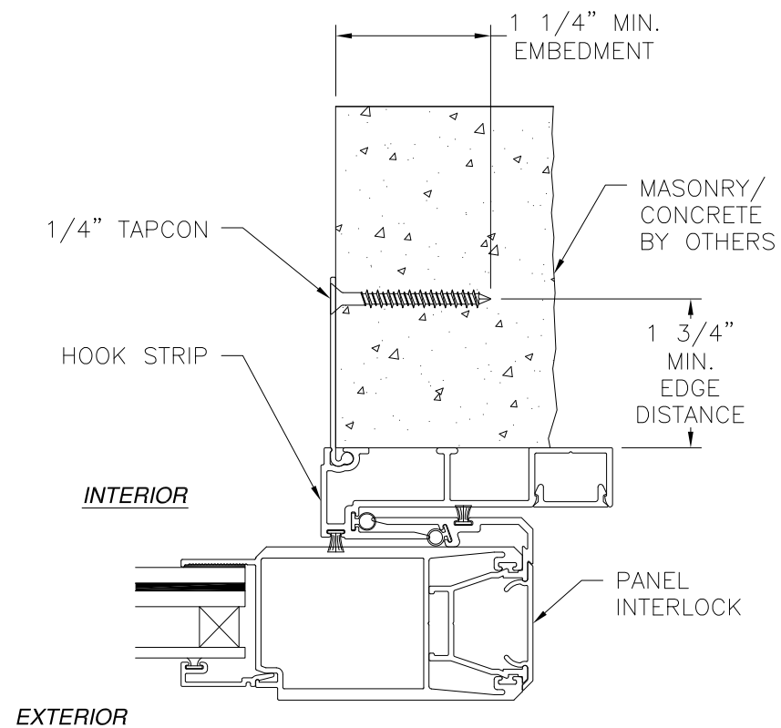
HOOK STRIP (M-2533) INSTALLATION MASONRY/CONCRETE
