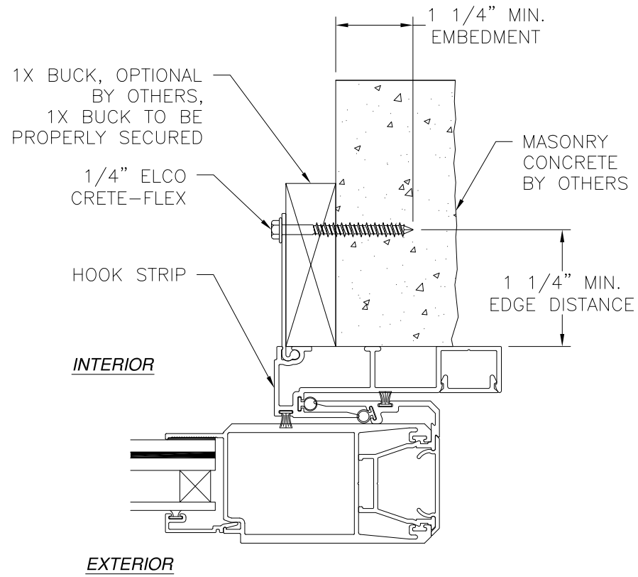
HOOK STRIP (M-2533) INSTALLATION MASONRY/CONCRETE
