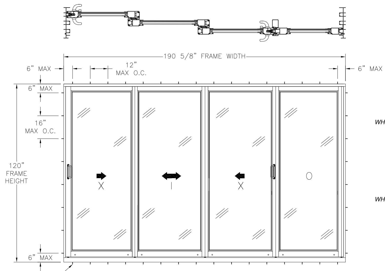
SERIES 120/130/140 ALUMINUM SGD - IMPACT EXTERIOR VIEW FINLESS & FLANGE INSTALLATION (4) PANELS SHOWN. UNLIMITED NUMBER OF PANELS IN UNLIMITED CONFIGURATIONS ARE APPROVED AS LONG AS INDIVIDUAL PANEL AREA DOES NOT EXCEED 40.49" FT 2
