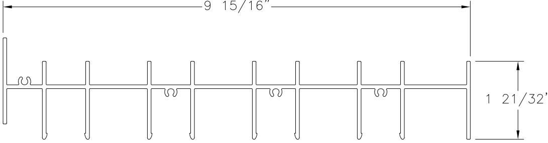
FRAME HEAD 4TRACK, FLANGE ALUMINUM 6005-T5 (M-2520)
