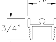
SILL SNAP-IN ROLLER TRACK ALUMINUM 6063-T5 (M-2511)
