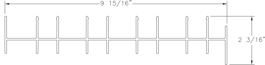
FRAME JAMB 4TRACK, FLANGE ALUMINUM 6005-T5 (M-2523)
