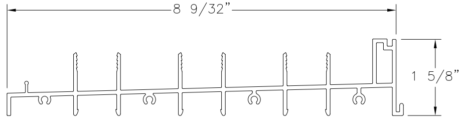
FRAME SILL 3TRACK ALUMINUM 6005-T5 (M-2522)
