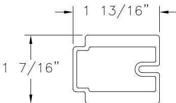
MEETING RAIL REINFORCEMENT ALUMINUM 6005-T5 (M-2516)
