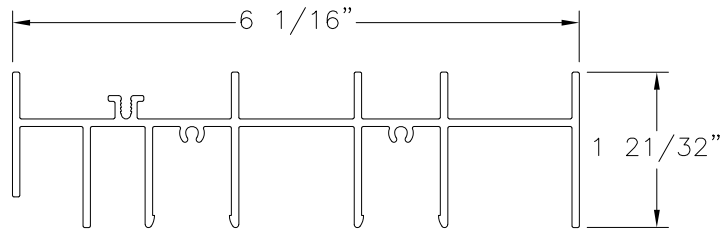
FRAME HEAD 2TRACK, FINLESS ALUMINUM 6005-T5 (M-2520)
