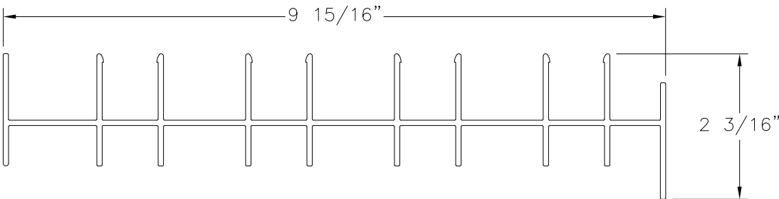
FRAME JAMB 4TRACK, FLANGE ALUMINUM 6005-T5 (M-2523)
