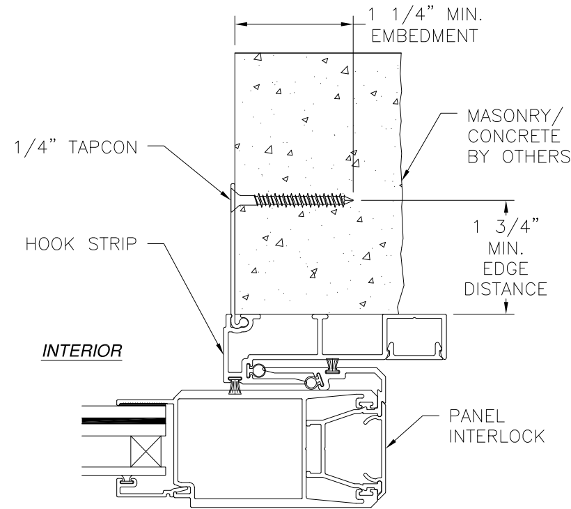
HOOK STRIP (M-2533) INSTALLATION MASONRY/CONCRETE
