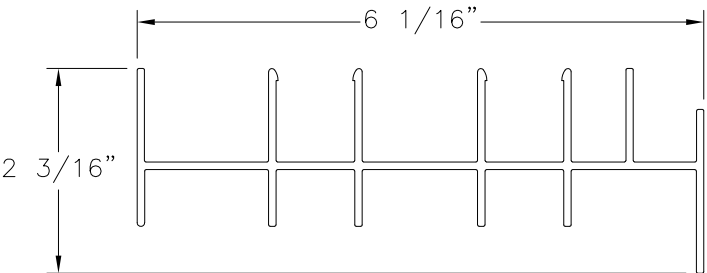
FRAME JAMB 2TRACK, FLANGE ALUMINUM 6005-T5 (M-2523)
