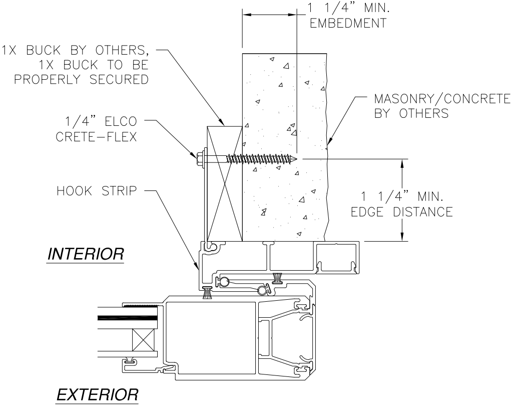
HOOK STRIP (M-2533) INSTALLATION MASONRY/CONCRETE
