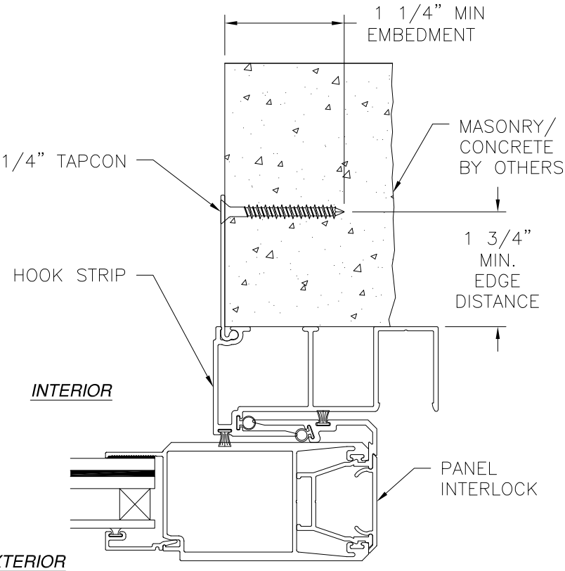
HOOK STRIP (M-2534) INSTALLATION MASONRY/CONCRETE
