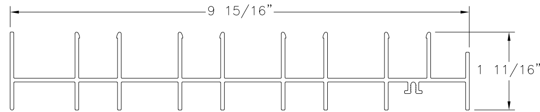
FRAME JAMB 4TRACK, FINLESS ALUMINUM 6005-T5 (M-2523)
