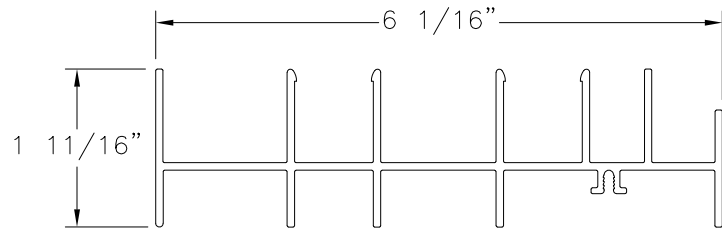
FRAME JAMB 2TRACK, FINLESS ALUMINUM 6005-T5 (M-2523)
