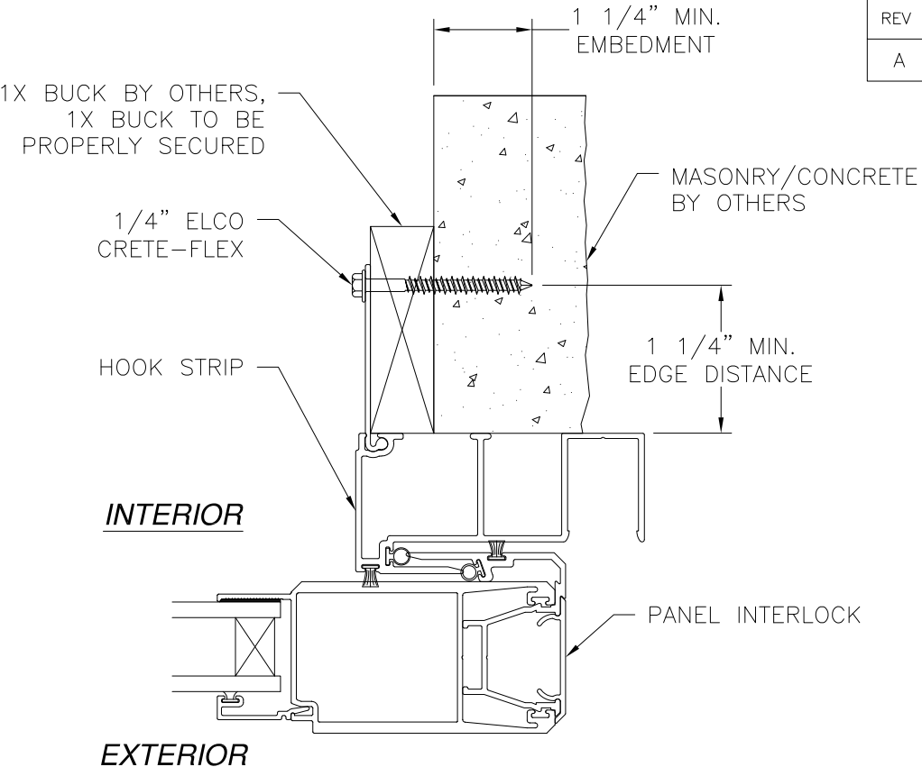
HOOK STRIP (M-2534) INSTALLATION MASONRY/CONCRETE
