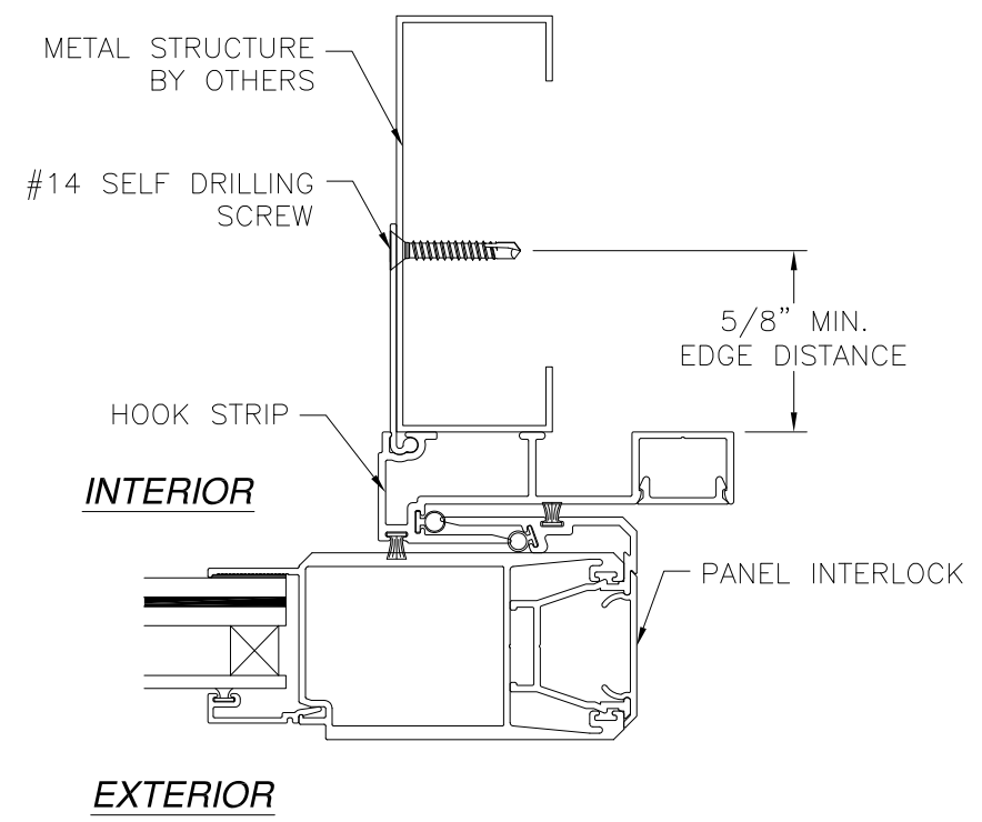
HOOK STRIP (M-2533) INSTALLATION METAL STRUCTURE
