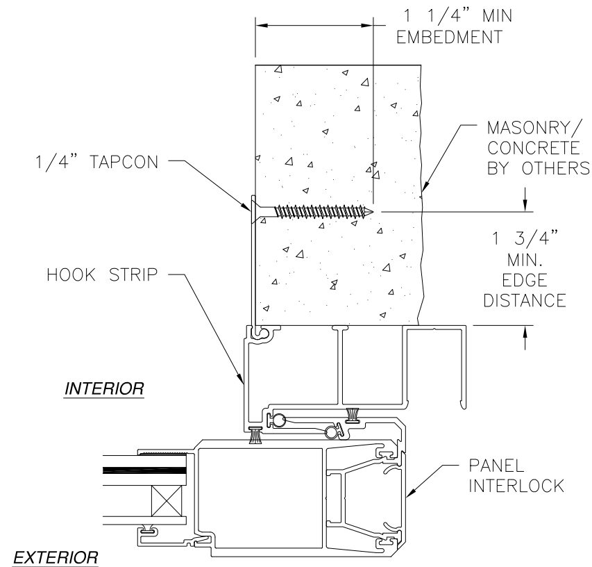
HOOK STRIP (M-2534) INSTALLATION MASONRY/CONCRETE
