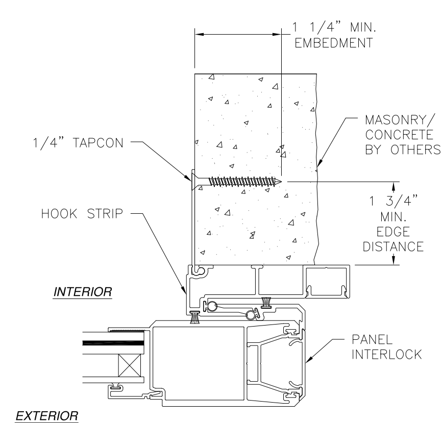
HOOK STRIP (M-2533) INSTALLATION MASONRY/CONCRETE
