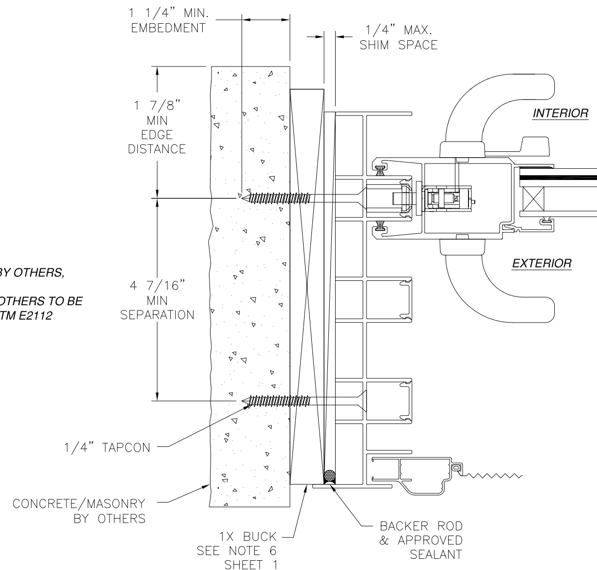
JAMB INSTALLATION DETAIL CONCRETE/MASONRY INSTALLATION
