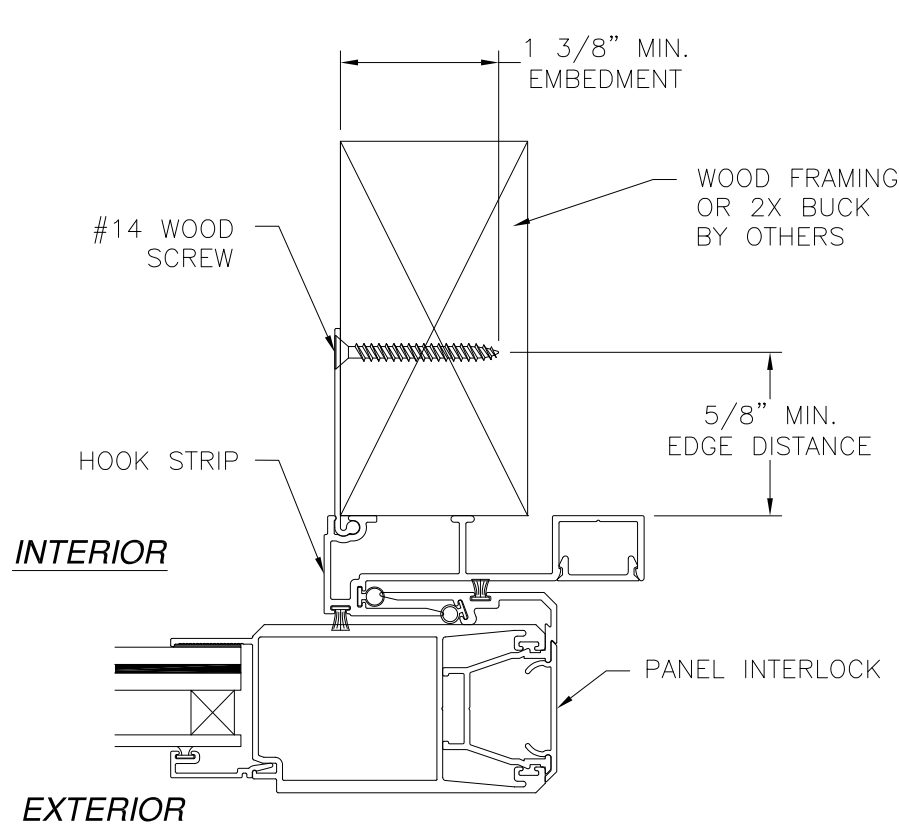
HOOK STRIP (M-2533) INSTALLATION 2X BUCK/WOOD FRAMING
