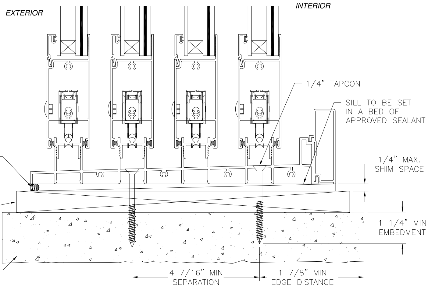
VERTICAL CROSS SECTION CONCRETE/MASONRY INSTALLATION
