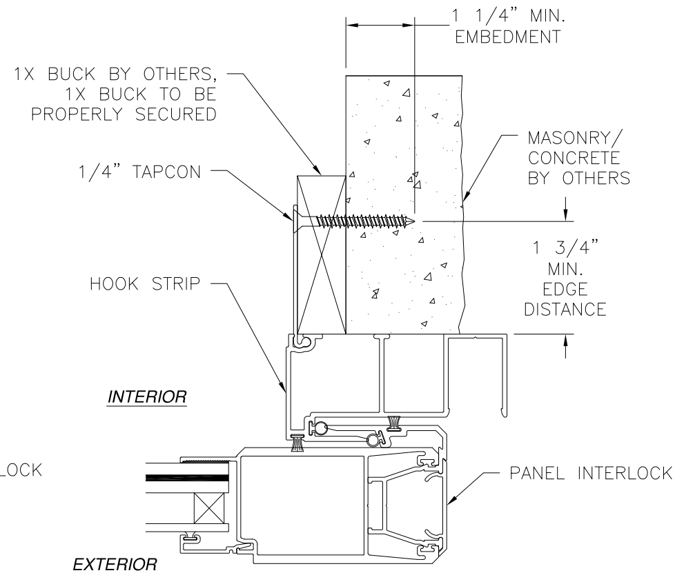
HOOK STRIP (M-2534) INSTALLATION MASONRY/CONCRETE
