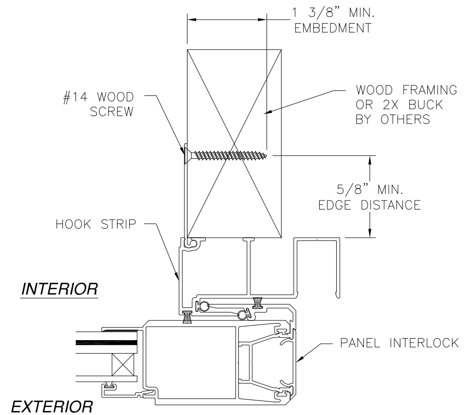
HOOK STRIP (M-2534) INSTALLATION 2X BUCK/WOOD FRAMING
