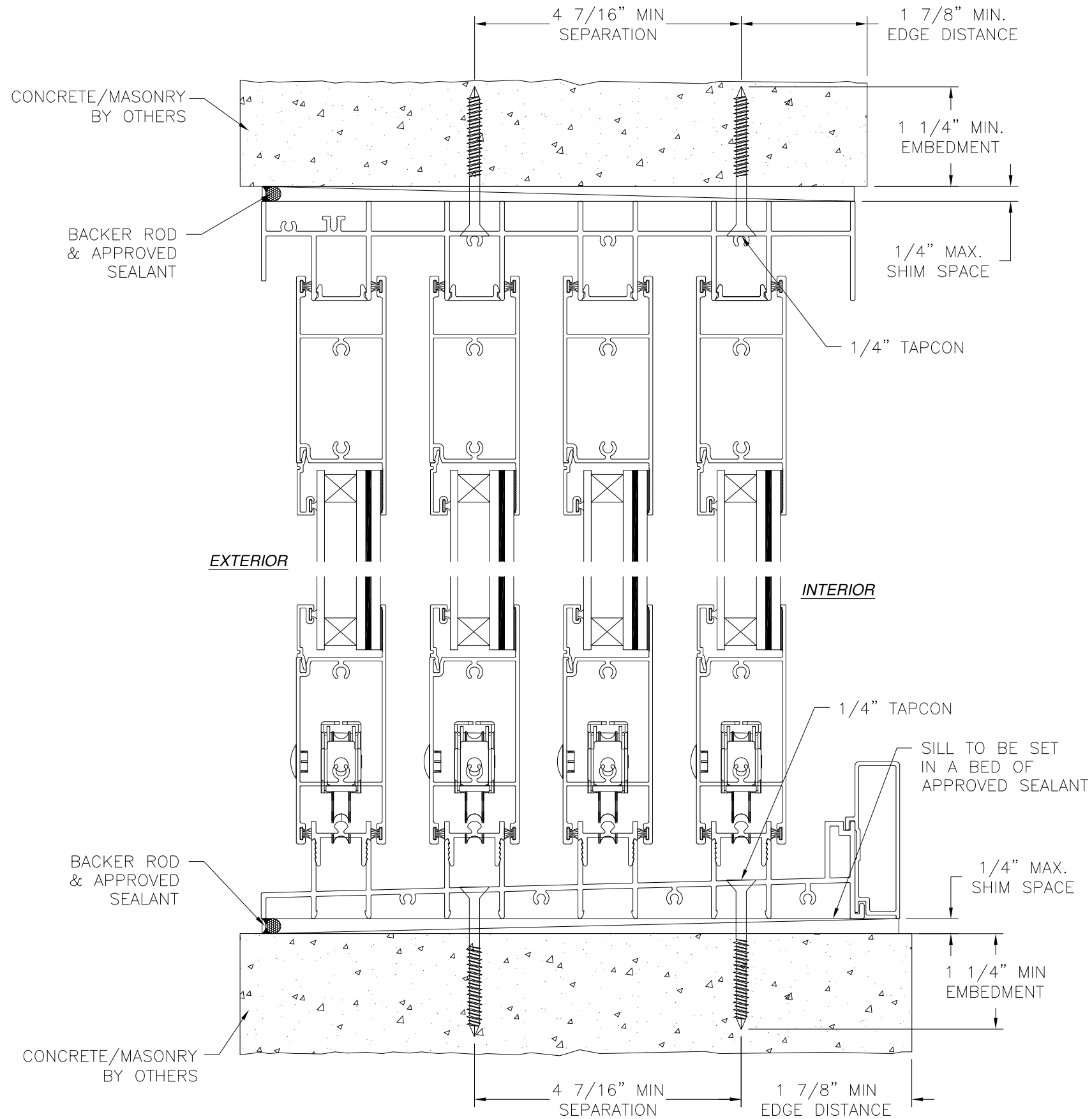
VERTICAL CROSS SECTION CONCRETE/MASONRY INSTALLATION HEAD AND SILL SHOWN, JAMBS SIMILAR
