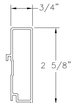
2 5/8" SILL EXTENDER ALUMINUM 6063-T5 .062" THICK
