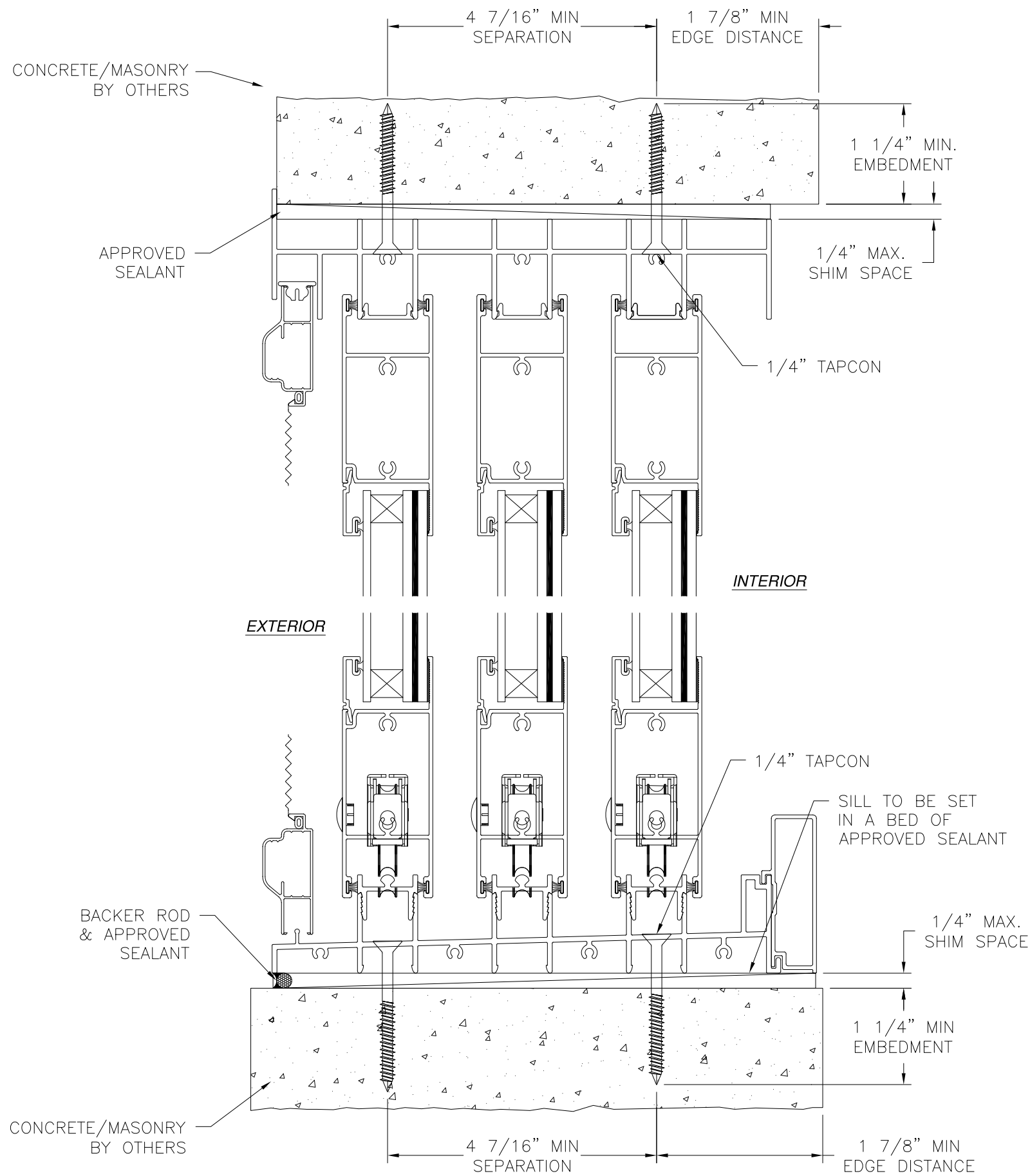
VERTICAL CROSS SECTION CONCRETE/MASONRY INSTALLATION HEAD AND SILL SHOWN, JAMBS SIMILAR
