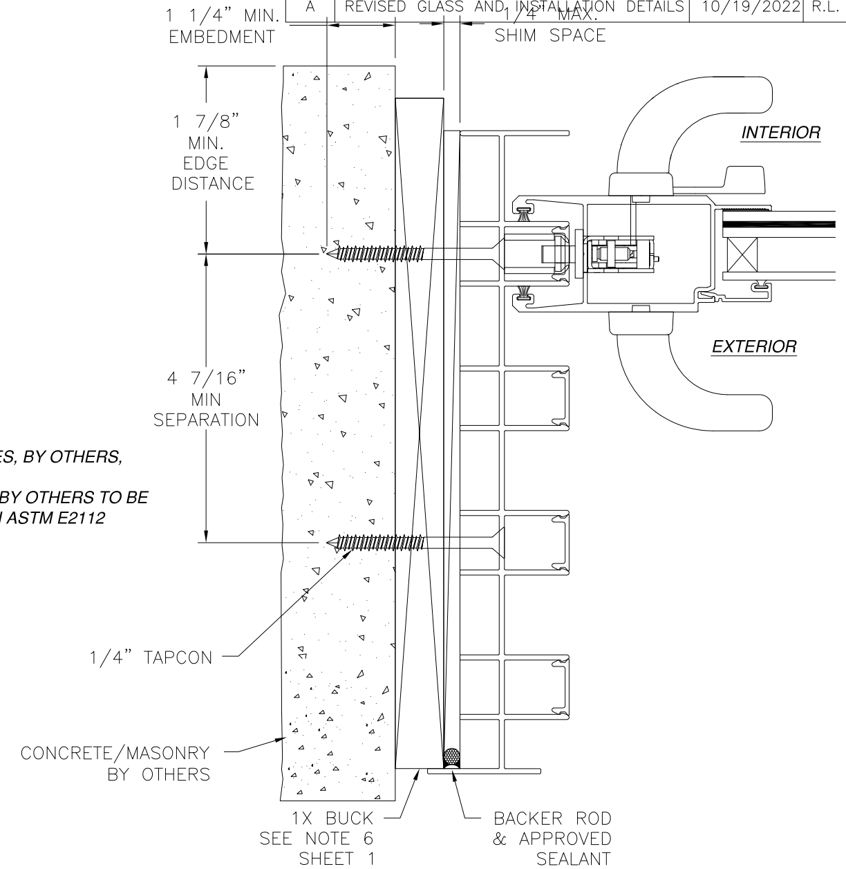
JAMB INSTALLATION DETAIL CONCRETE/MASONRY INSTALLATION
