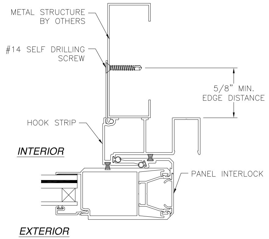
HOOK STRIP (M-2534) INSTALLATION METAL STRUCTURE
