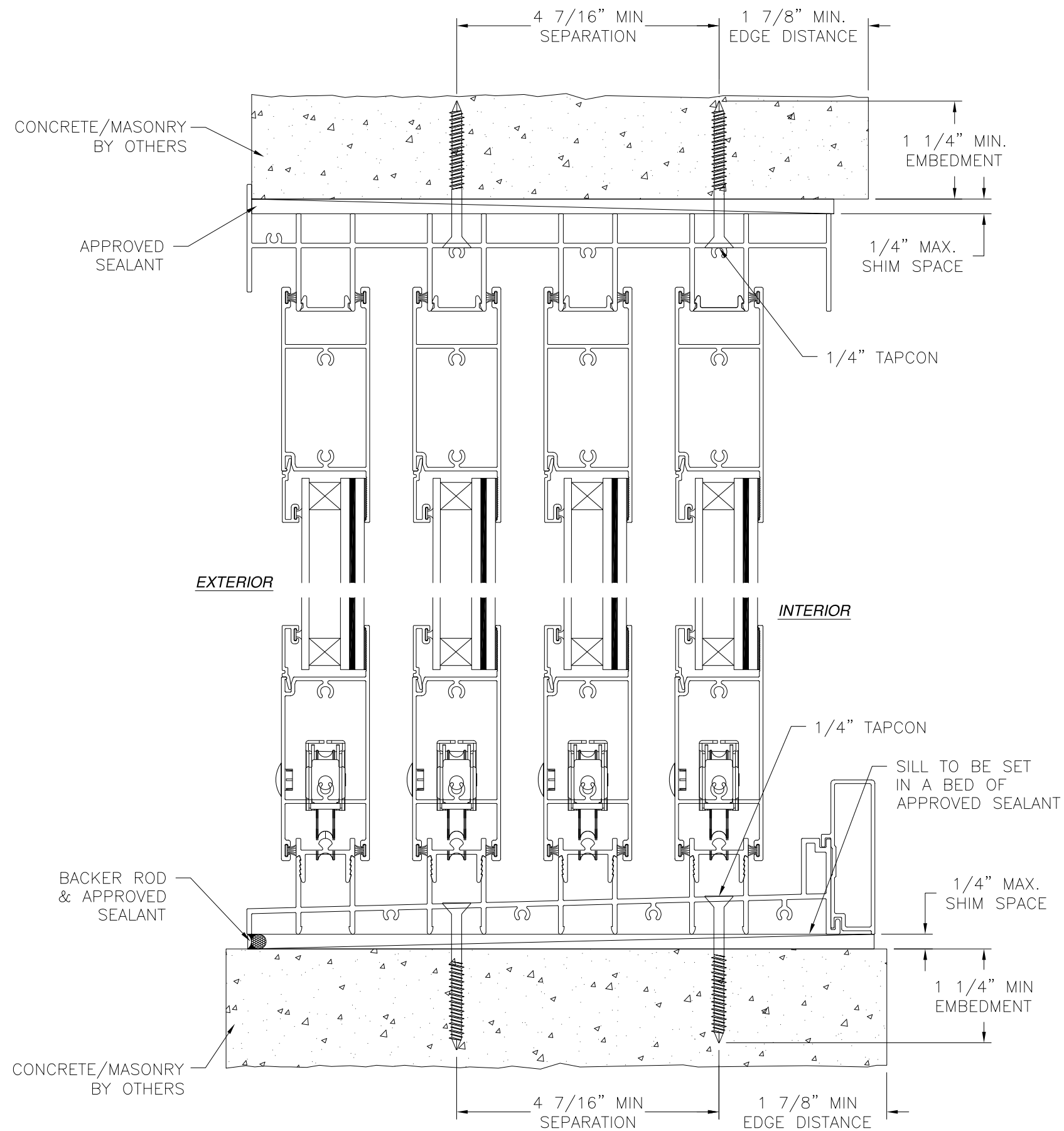
VERTICAL CROSS SECTION CONCRETE/MASONRY INSTALLATION HEAD AND SILL SHOWN, JAMBS SIMILAR
