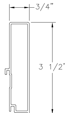
3 1/2" SILL EXTENDER ALUMINUM 6063-T5 .062" THICK
