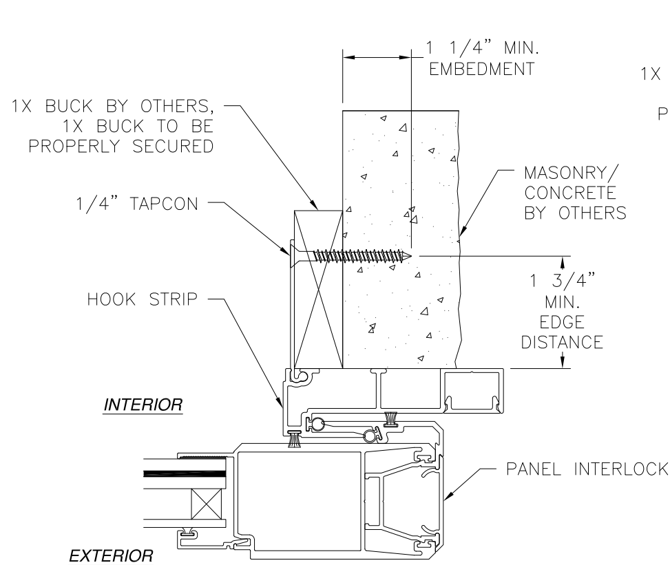
HOOK STRIP (M-2533) INSTALLATION MASONRY/CONCRETE
