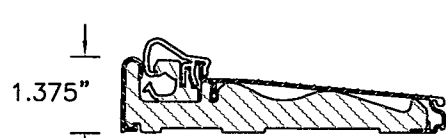
ZAC I/S THRESHOLD
