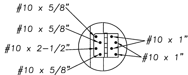
DETAIL "C"
