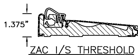
INSWING THRESHOLD
