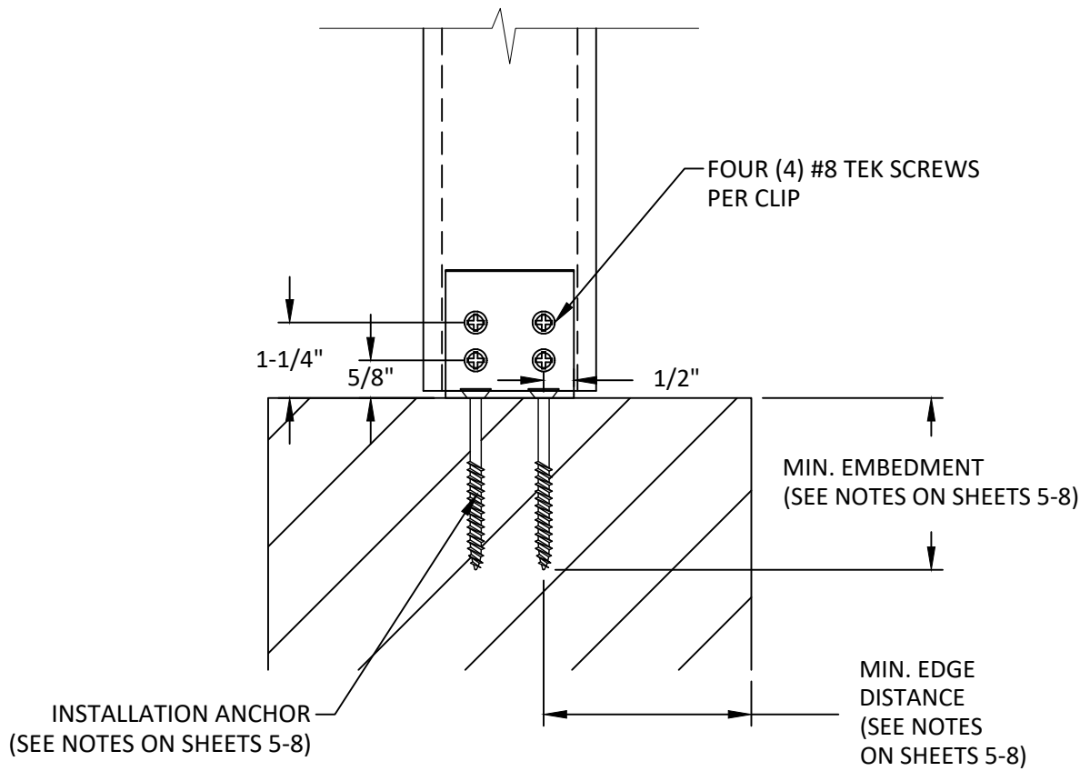
A 2 SIDE VIEW MULLION W/ END CLIPS (ONE OR TWO WAY) STANDARD CLIP
