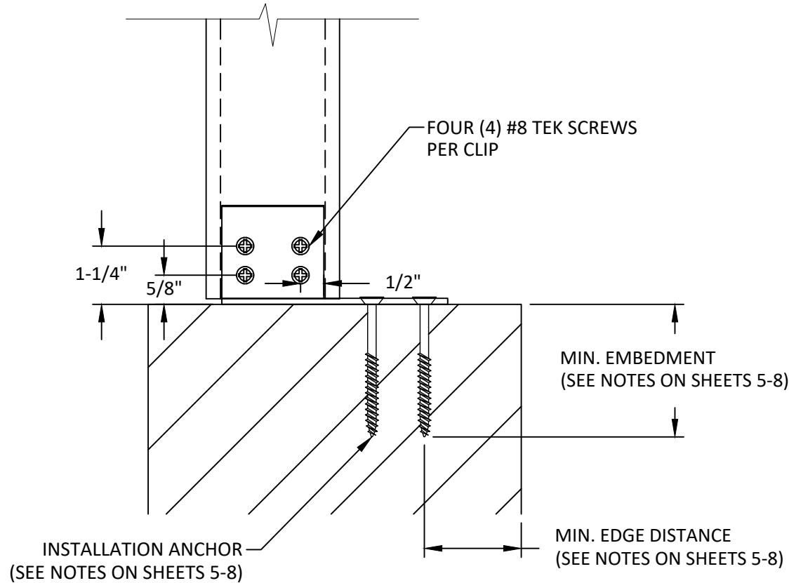
F 3 SIDE VIEW MULLION W/ END CLIPS (ONE OR TWO WAY) OFFSET CLIP
