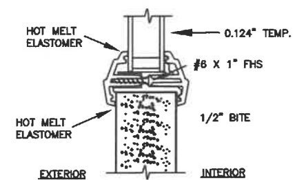
ALTERNATE GLAZING DETAIL NON-IMPACT GLASS
