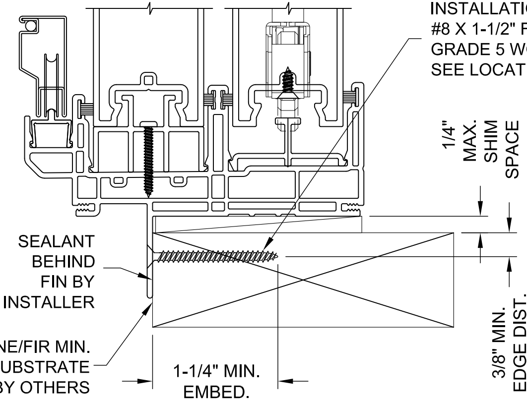
TYPICAL FRAME VERTICAL SECTION
