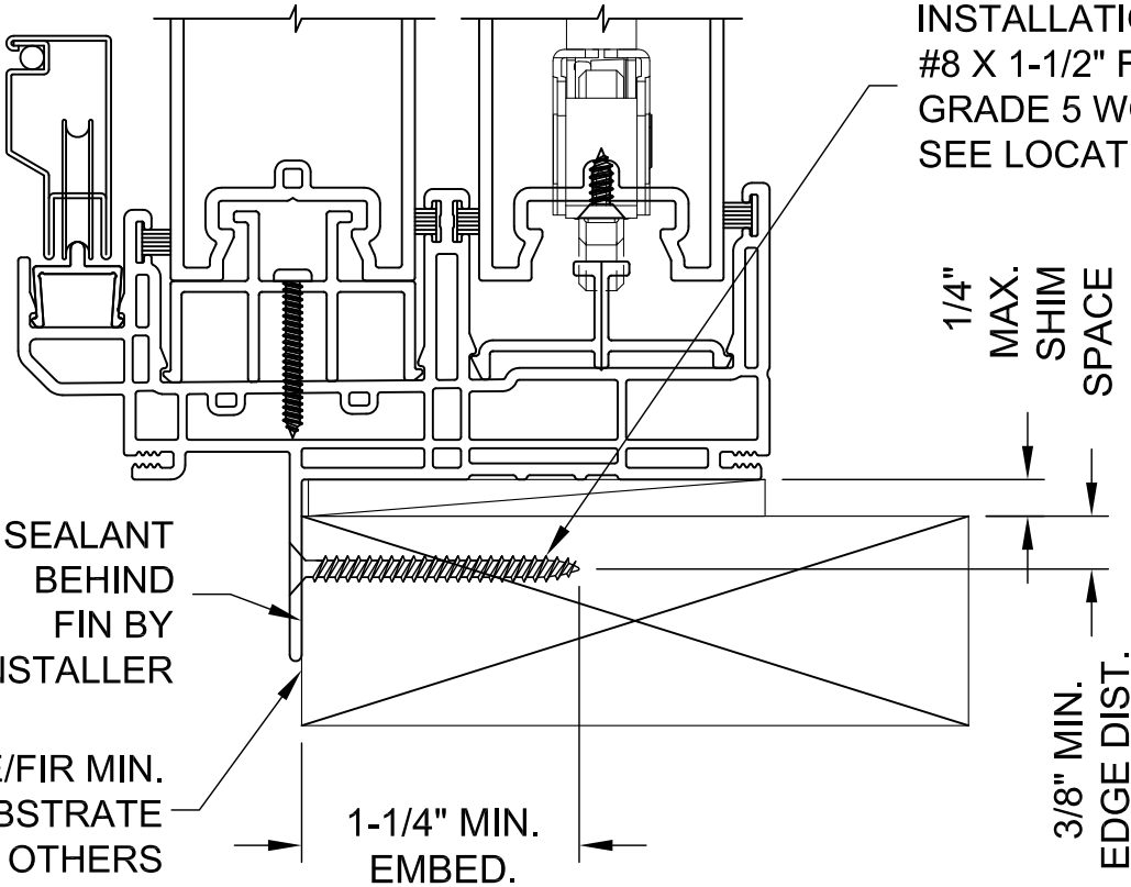
TYPICAL FRAME VERTICAL SECTION
