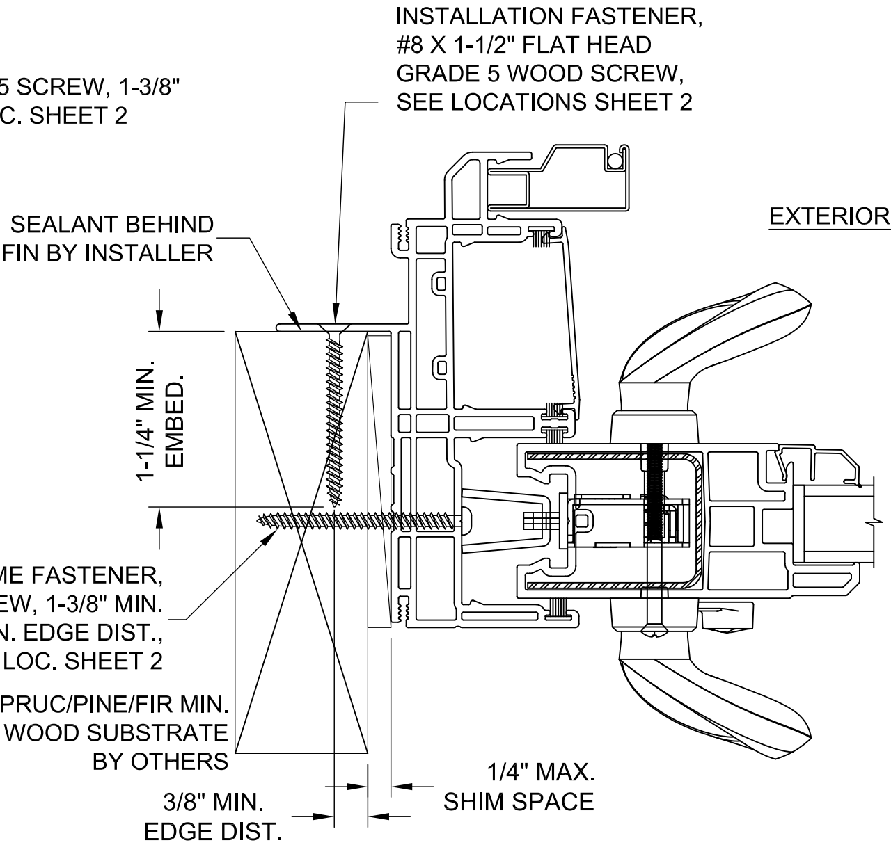
TYPICAL JAMB HORIZONTAL SECTION (LOCK JAMB SHOWN, FIXED JAMB ANCHORAGE SIMILAR)
