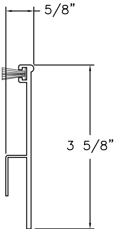
SILL RISER ALUMINUM
