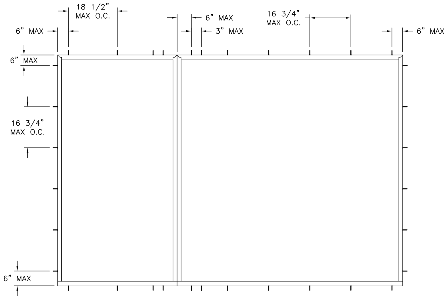
ANCHORING LAYOUT
