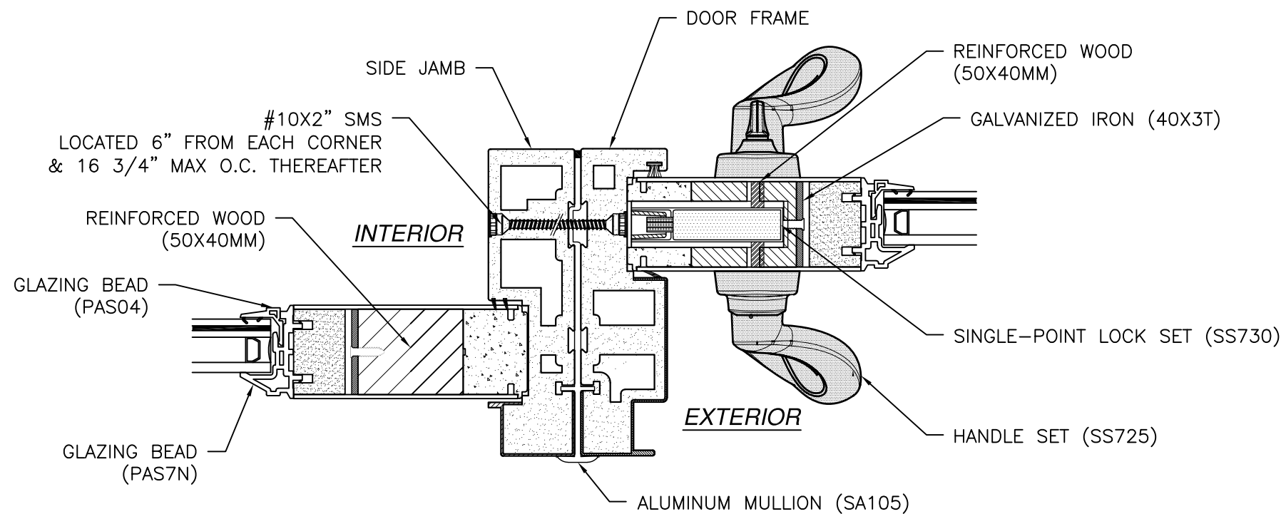
MULLION DETAIL
