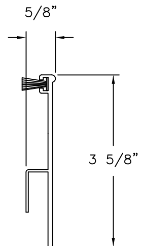
SILL RISER ALUMINUM
