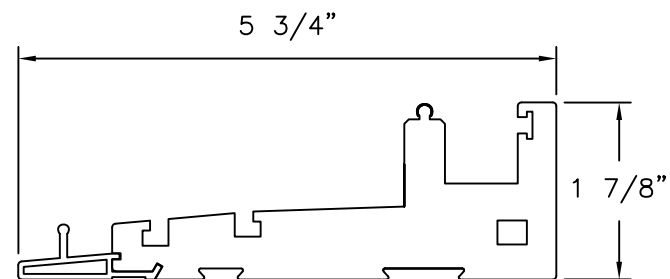
SILL FOAM PVC & ALUMINUM
