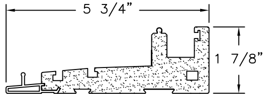
SILL FOAM PVC & ALUMINUM
