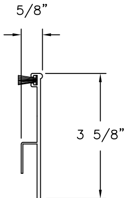
SILL RISER ALUMINUM
