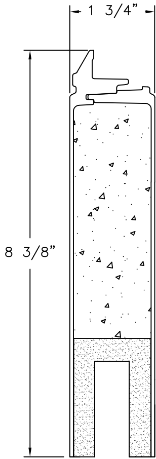
OPERABLE PANEL BOTTOM RAIL PAS7F, PVC FOAM
