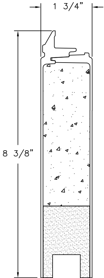
FIXED PANEL BOTTOM RAIL PAS7F, PVC FOAM
