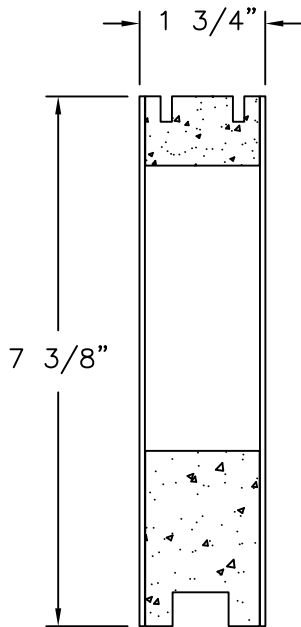
FIXED PANEL BOTTOM RAIL FOAM PVC
