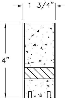
OPERABLE AND FIXED PANEL TOP RAIL FOAM PVC
