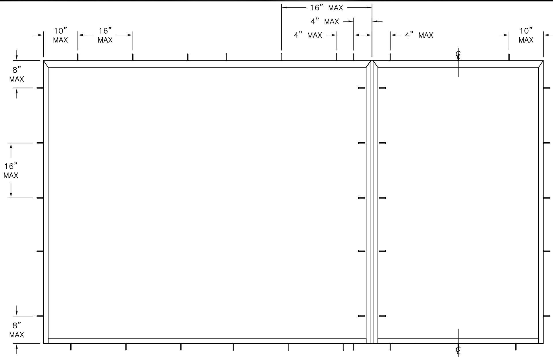
SRS GLIDING PATIO DOOR ANCHORING LAYOUT
