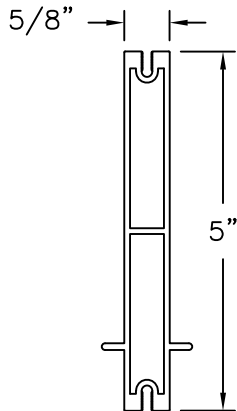
MULLION ALUMINUM 6063-T5 (.078" THICK)
