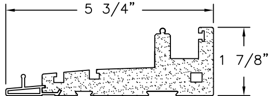
SILL FOAM PVC & ALUMINUM
