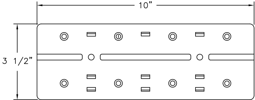
PLATE STAINLESS STEEL
