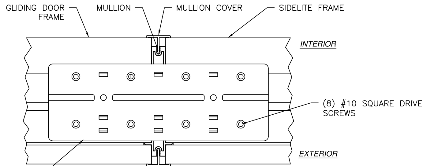
CONNECTION PLATE MULLION CONNECTION DETAIL
