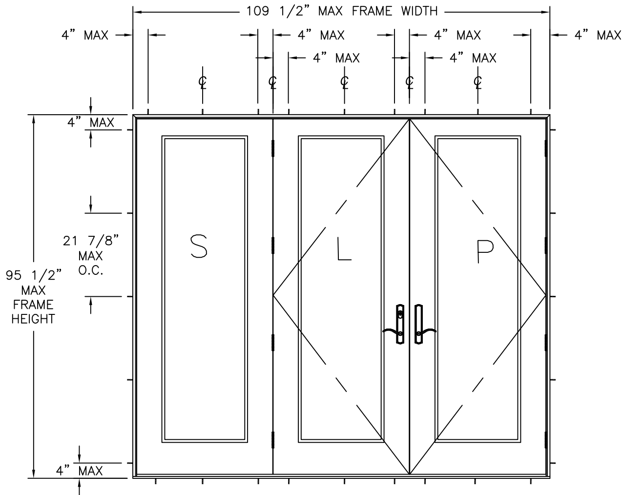
8' OUTSWING DOOR SLP (OXX) EXTERIOR VIEW
