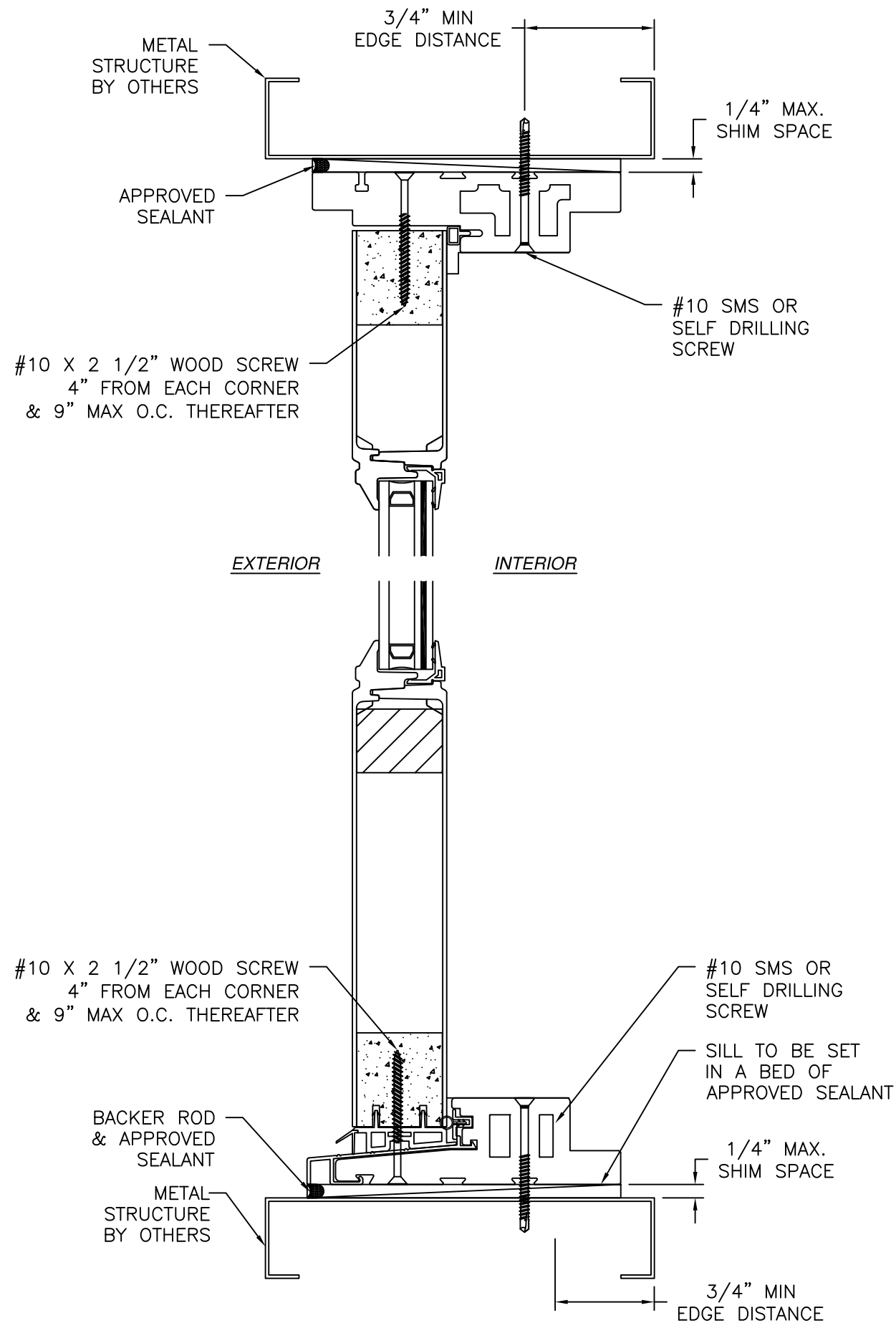
VERTICAL CROSS SECTION METAL STRUCTURE INSTALLATION
