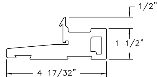
INSWING SILL FOAM PVC CO-EX
