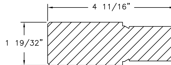
MULLION REINFORCEMENT WHITE PINE
