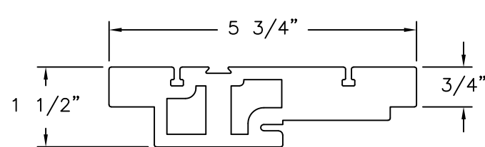
HEAD FRAME & JAMB FOAM PVC CO-EX
