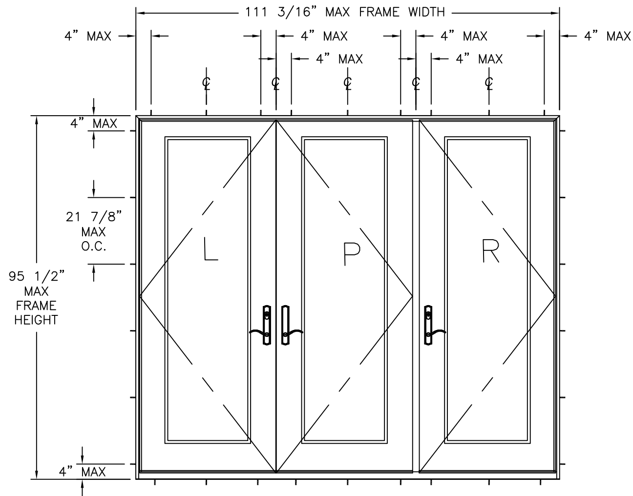
8' INSWING DOOR LPR (X/XX) EXTERIOR VIEW
