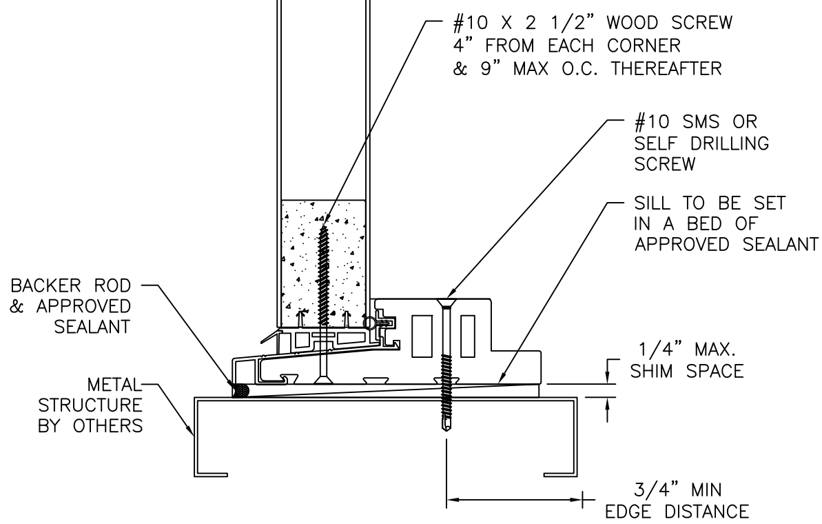
VERTICAL CROSS SECTION METAL STRUCTURE INSTALLATION
