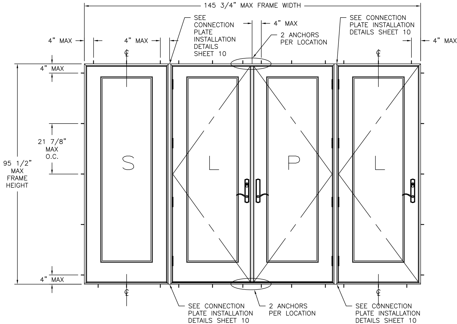
SERIES SLPL GLAZED OUTSWING DOOR EXTERIOR VIEW
