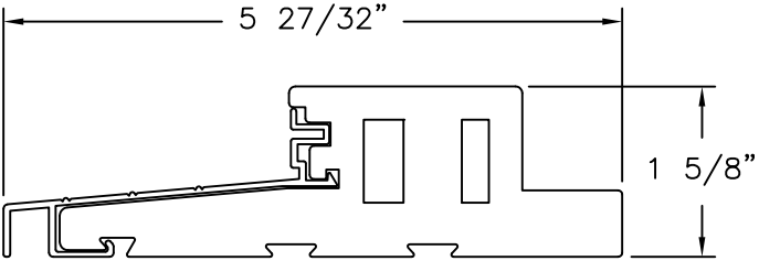
OUTSWING SILL FOAM PVC CO-EX & ALUMINUM
