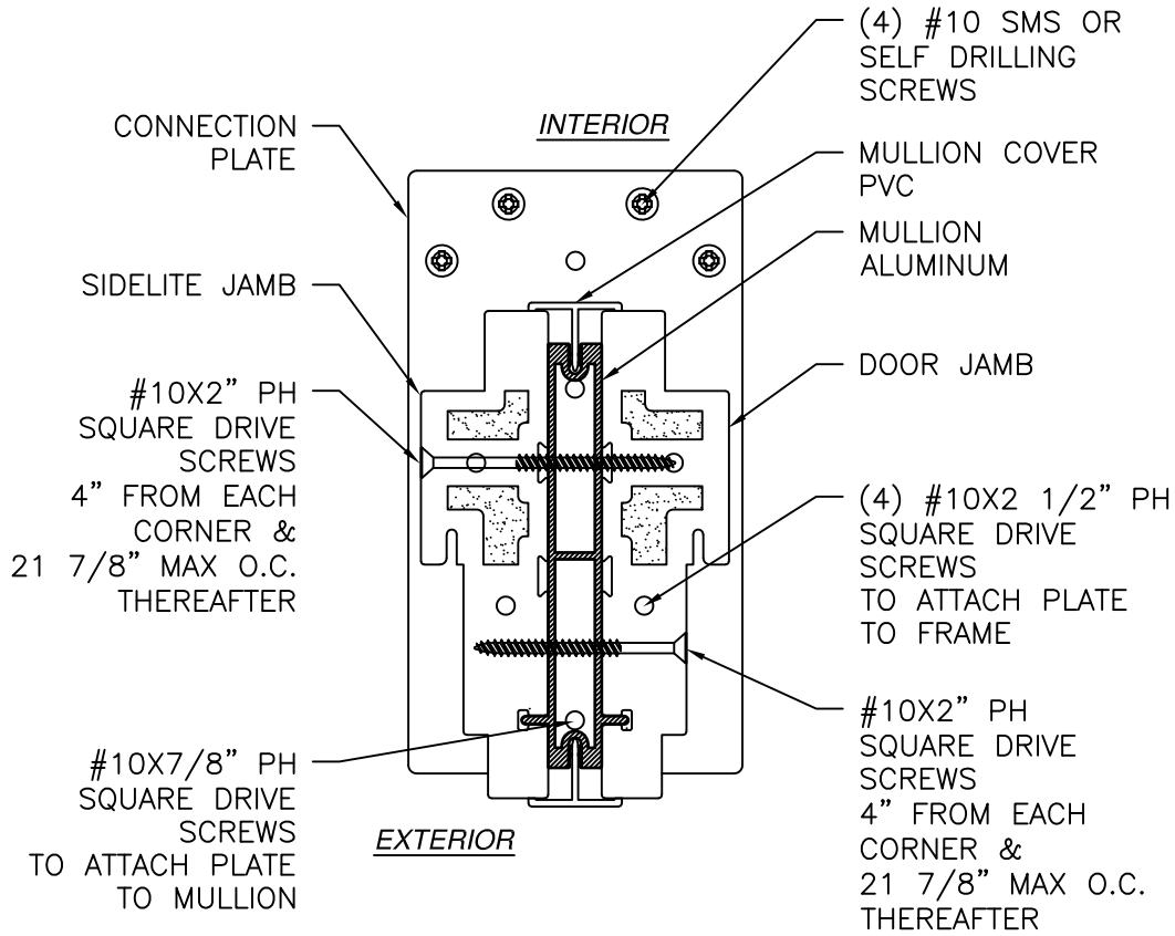
CONNECTION PLATE METAL STRUCTURE INSTALLATION
