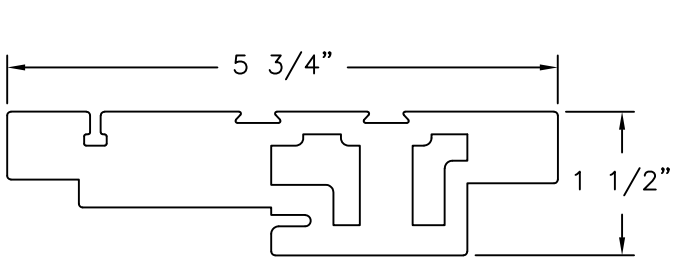
HEAD FRAME & JAMB FOAM PVC CO-EX
