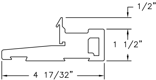
INSWING SILL FOAM PVC CO-EX
