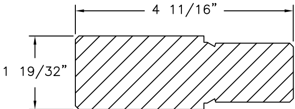
MULLION REINFORCEMENT WHITE PINE
