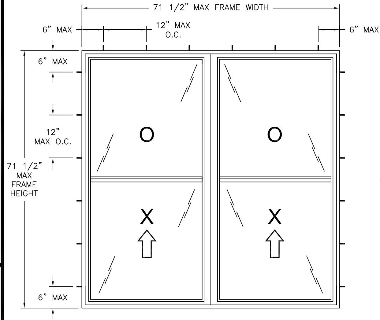
SERIES 900/950 CHS TWIN MULLED VINYL SH EXTERIOR VIEW FRAME INSTALLATION
