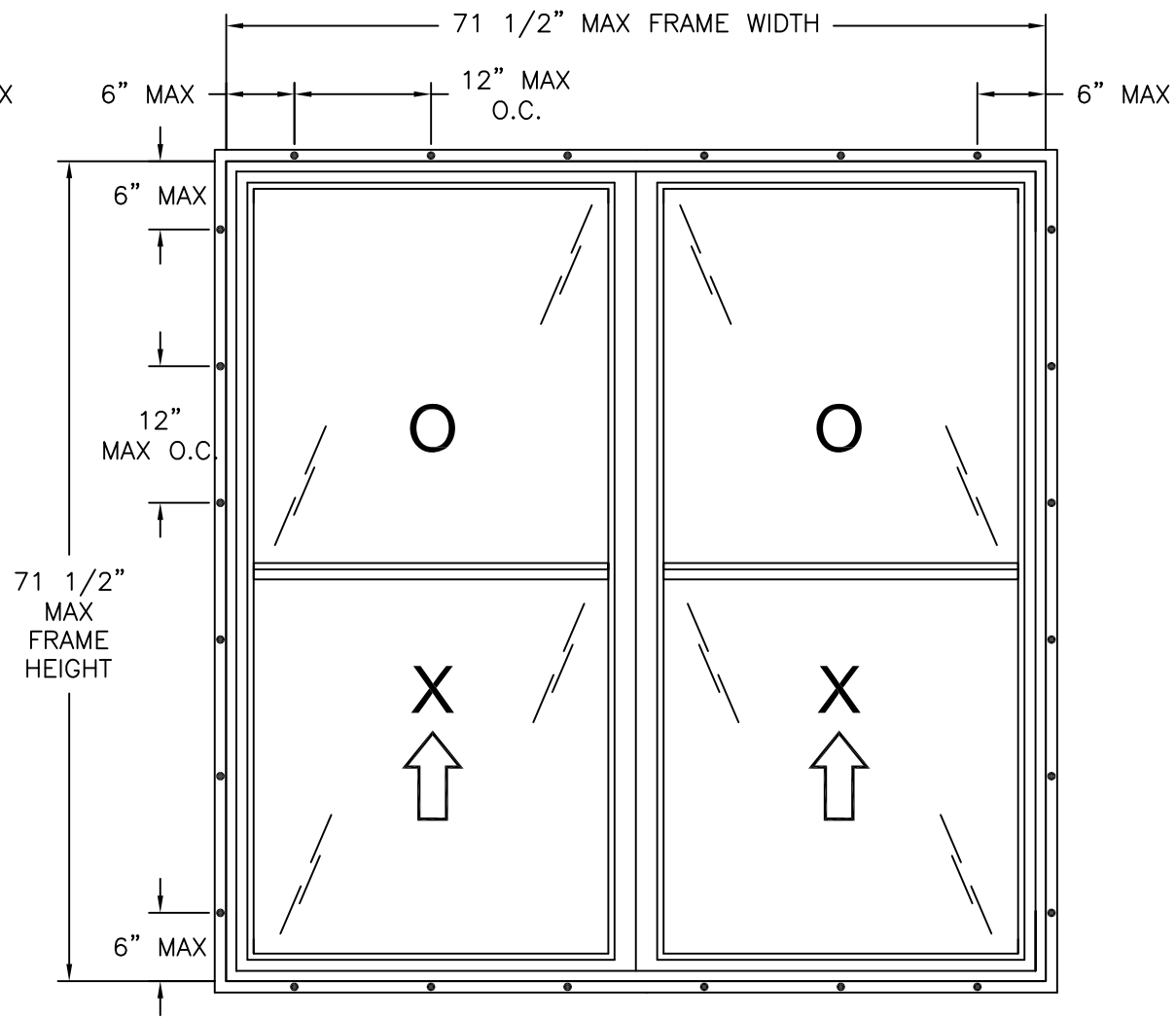
SERIES 900/950 CHS TWIN MULLED VINYL SH EXTERIOR VIEW FIN INSTALLATION
