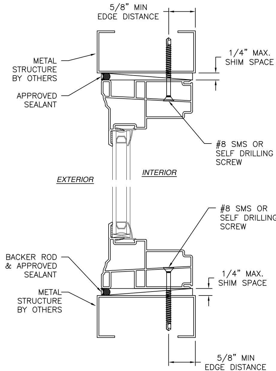
VERTICAL CROSS SECTION METAL STRUCTURE INSTALLATION
