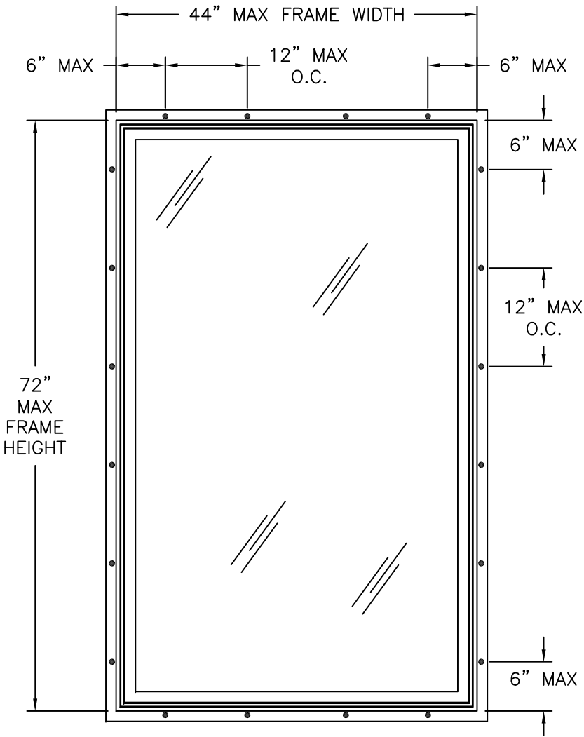
SERIES 901/951 VINYL FIXED WINDOW EXTERIOR VIEW FIN INSTALLATION
