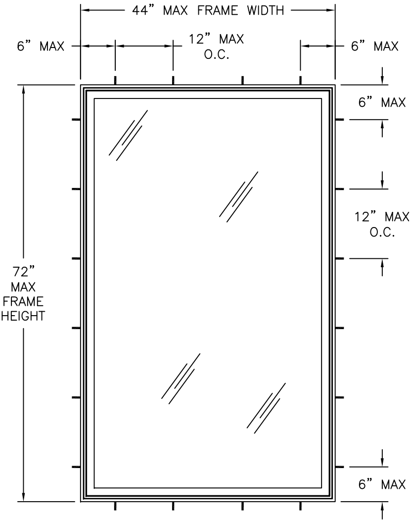
SERIES 901/951 VINYL FIXED WINDOW EXTERIOR VIEW FRAME INSTALLATION
