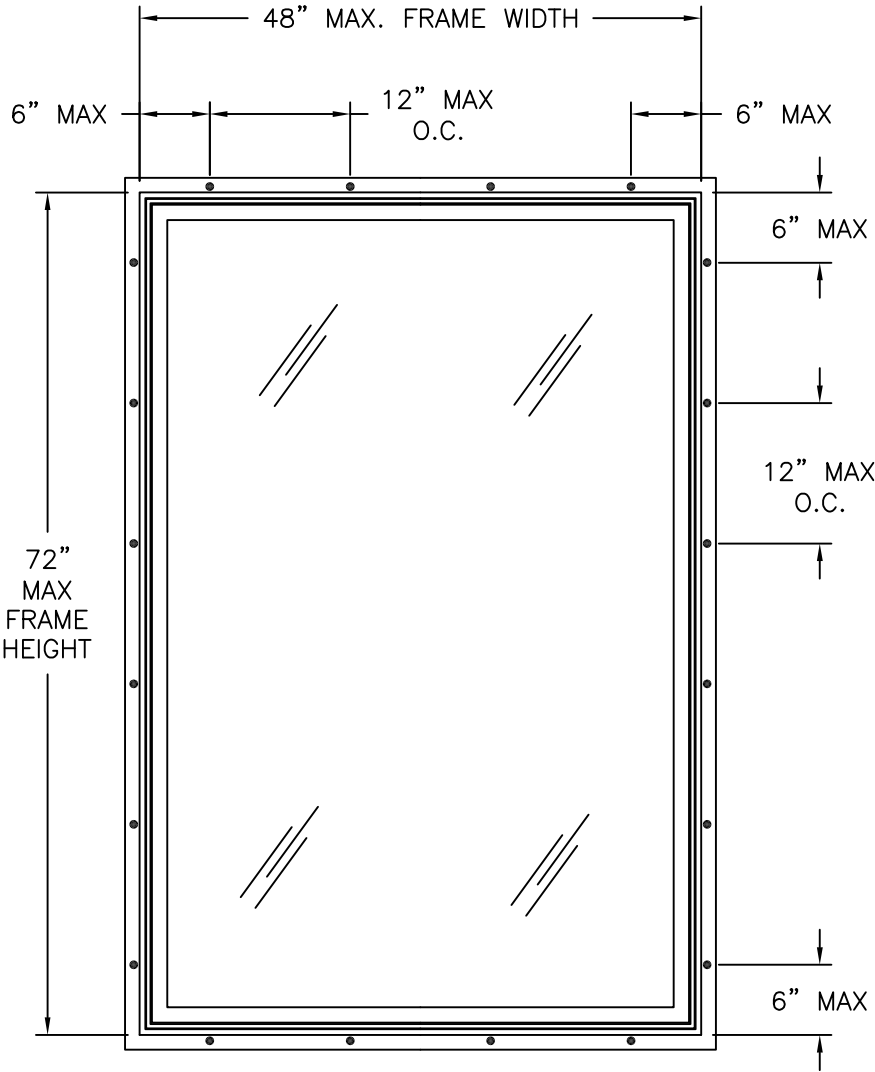
SERIES 901/951 VINYL FIXED PICTURE WINDOW EXTERIOR VIEW FIN INSTALLATION
