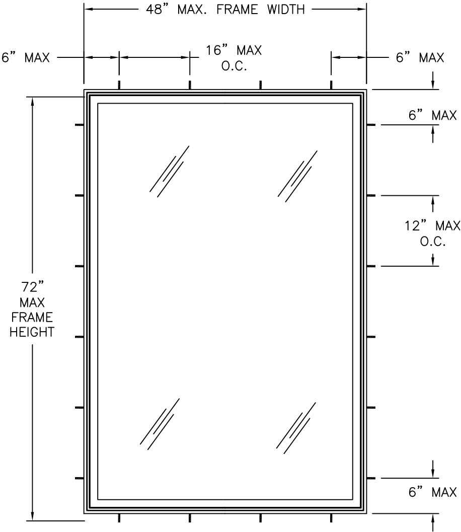
SERIES 901/951 VINYL FIXED PICTURE WINDOW EXTERIOR VIEW FRAME INSTALLATION
