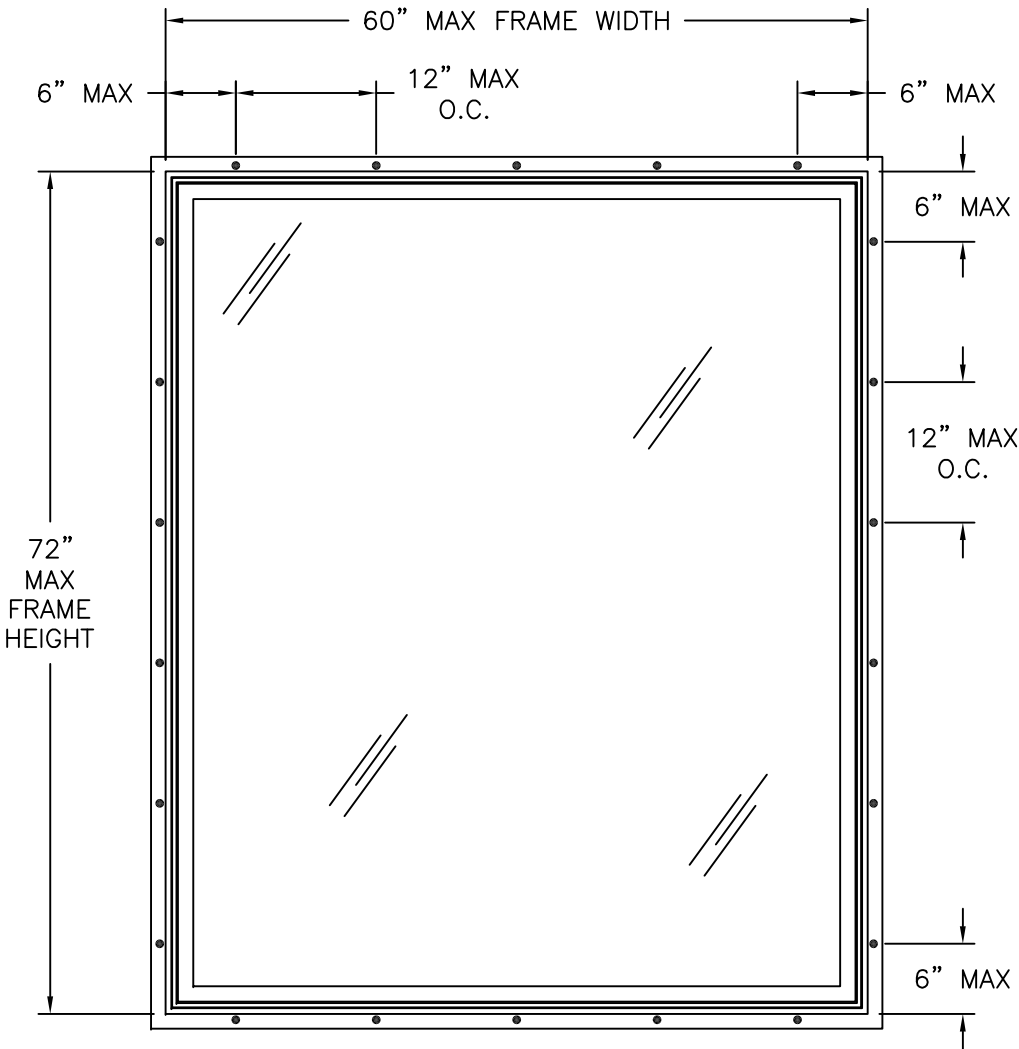
SERIES 901/951 VINYL FIXED PICTURE WINDOW EXTERIOR VIEW FIN INSTALLATION
