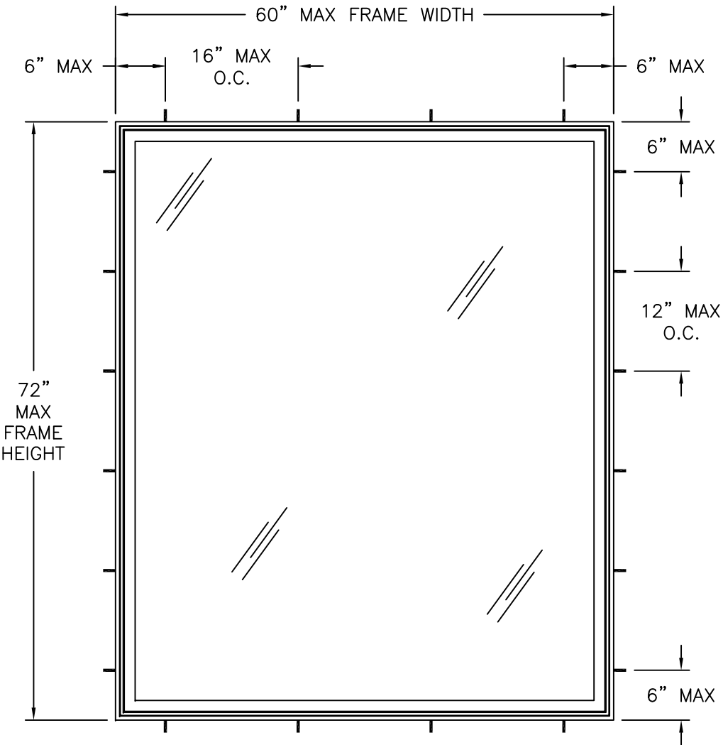
SERIES 901/951 VINYL FIXED PICTURE WINDOW EXTERIOR VIEW FRAME INSTALLATION
