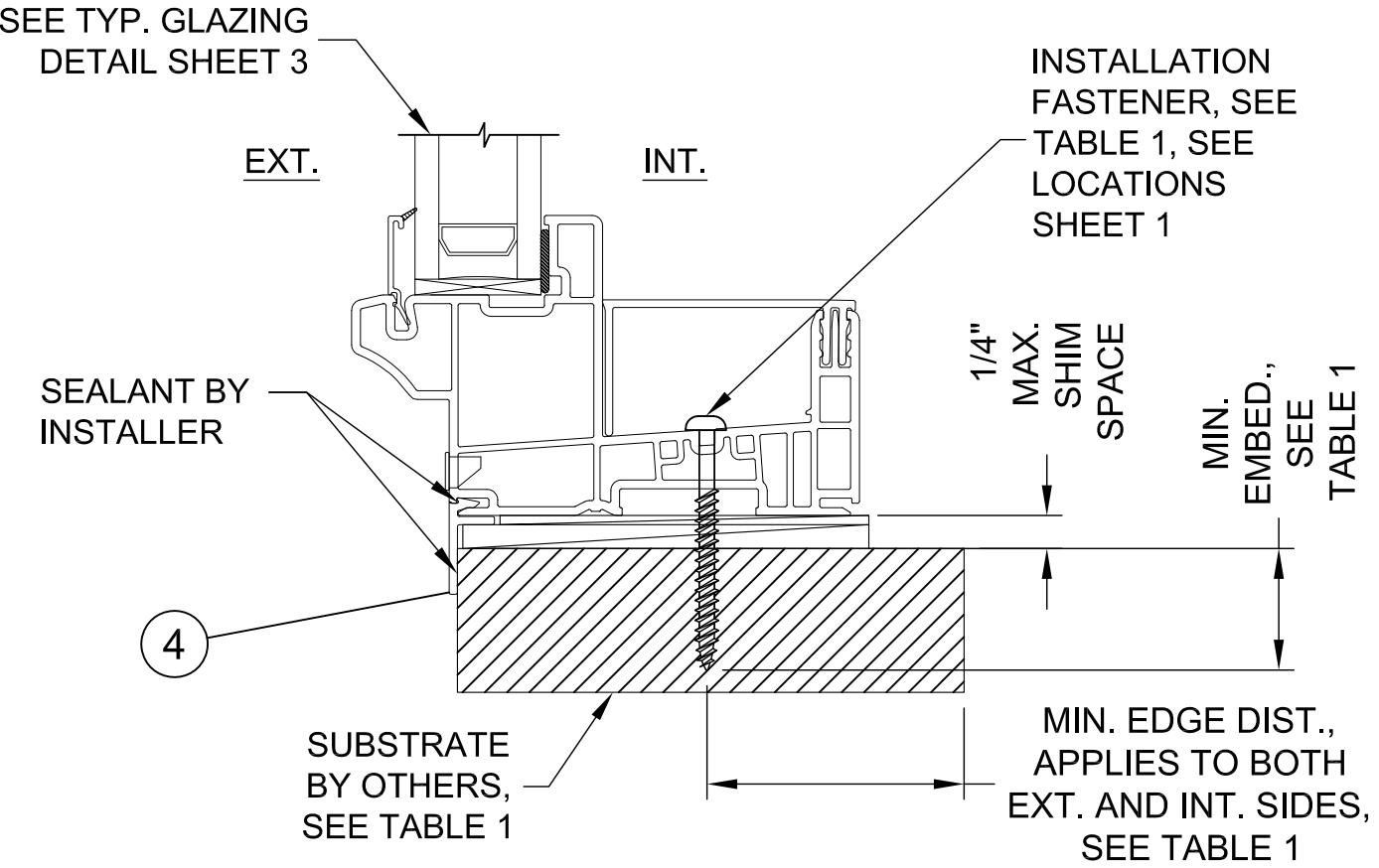
TYPICAL FLANGE INSTALLATION HEAD / SILL / JAMB
