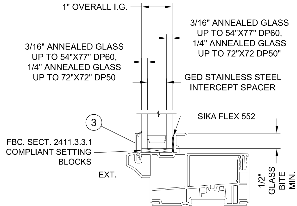
TYPICAL GLAZING DETAIL
