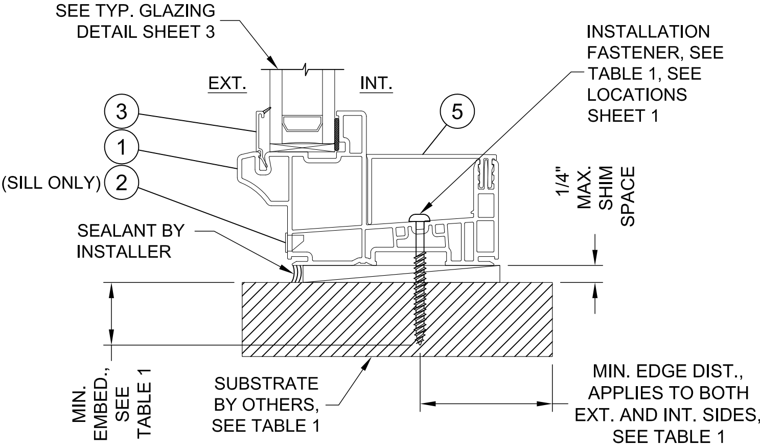
TYPICAL EQUAL LEG INSTALLATION HEAD / SILL / JAMB
