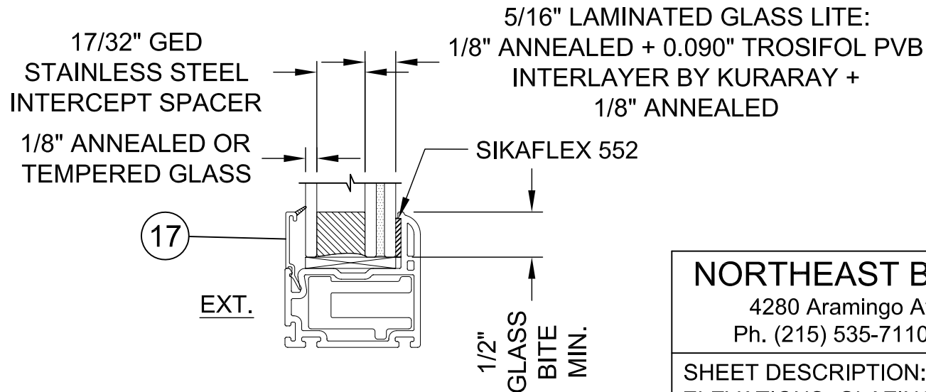
TYPICAL GLAZING DETAIL
