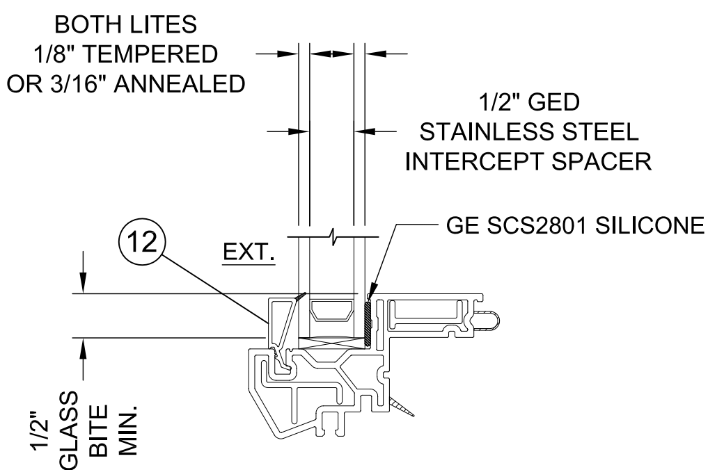
TYPICAL GLAZING DETAIL
