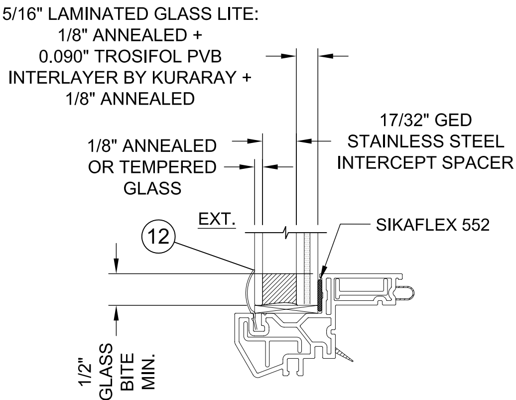
TYPICAL GLAZING DETAIL
