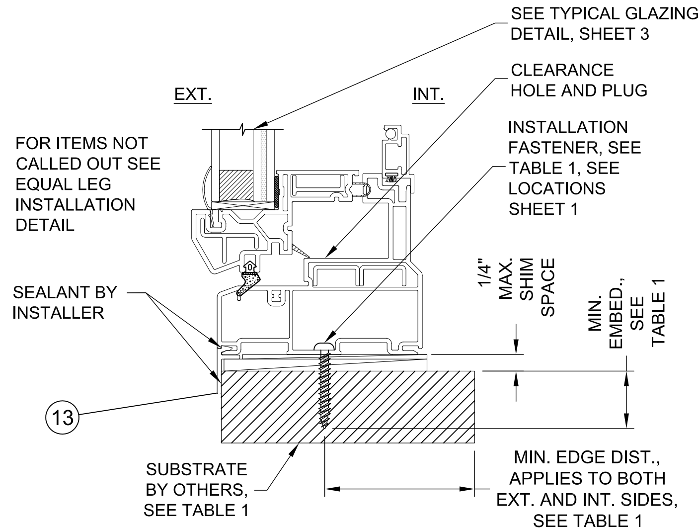
TYPICAL FLANGE INSTALLATION HEAD / SILL / JAMB
