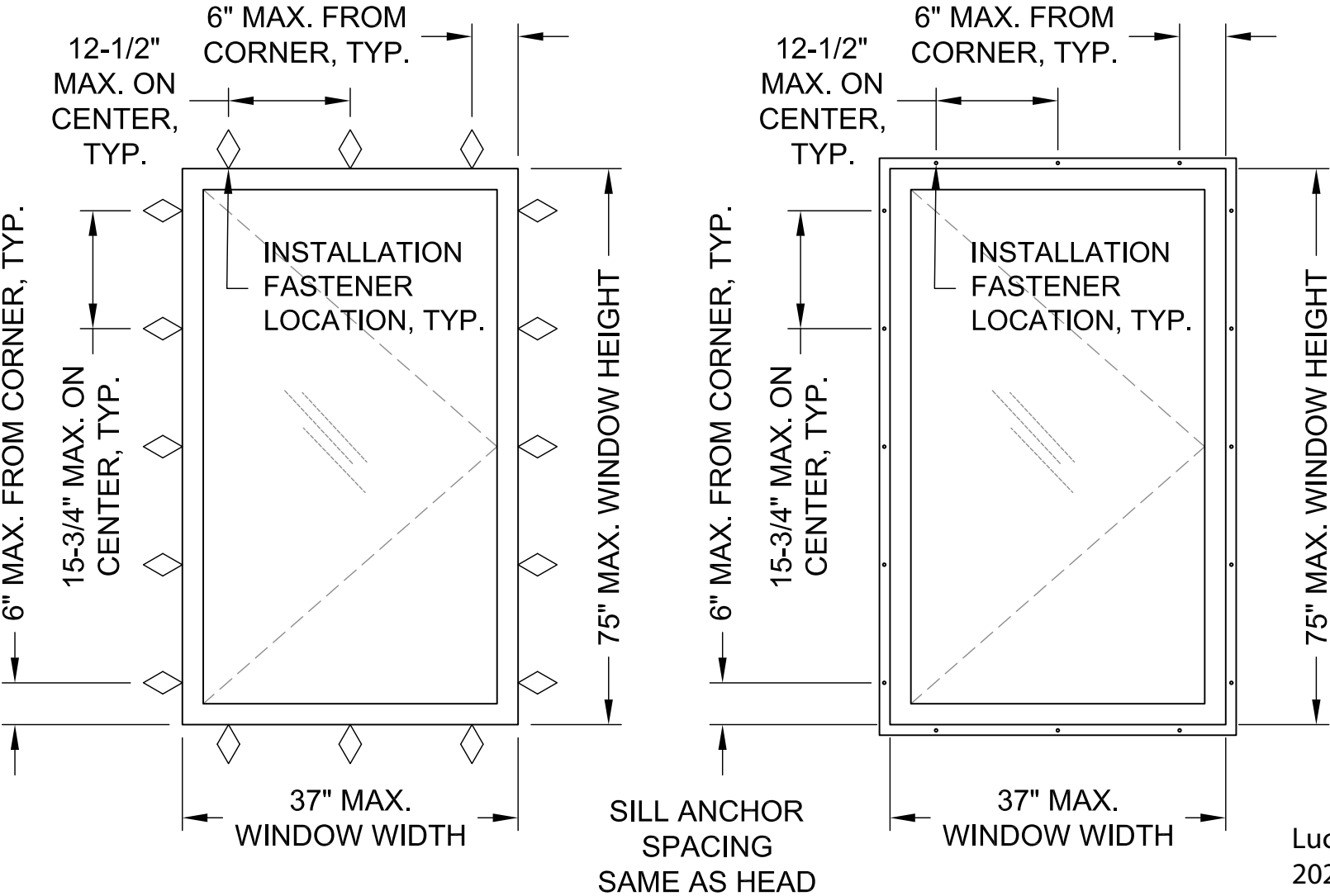
EQUAL LEG / FLANGE ELEVATION SEE DETAILS SHEET 2 FIN ELEVATION SEE DETAILS SHEET 3
