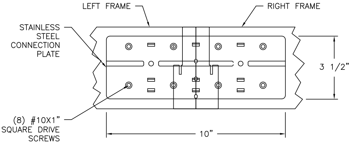
FRAME CONNECTION DETAIL
