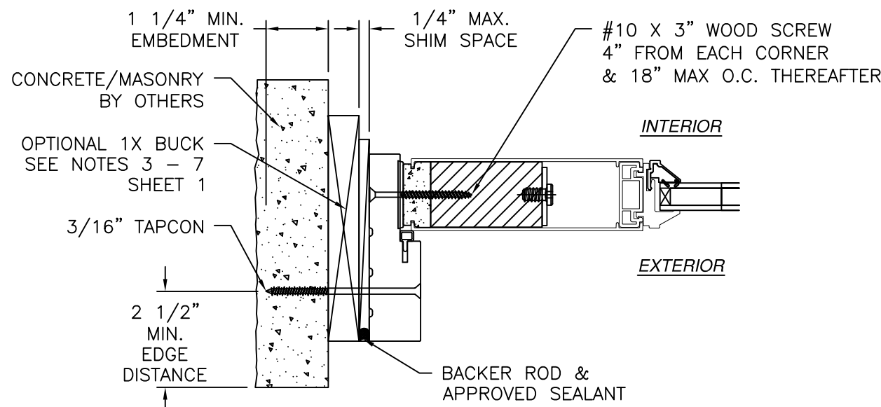
JAMB INSTALLATION DETAIL CONCRETE/MASONRY INSTALLATION
