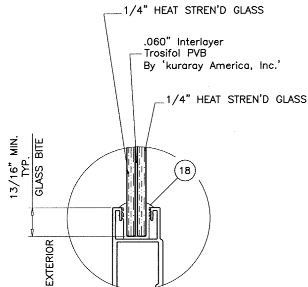
GLAZING DETAIL 9/16" OVERALL LAM. GLASS
