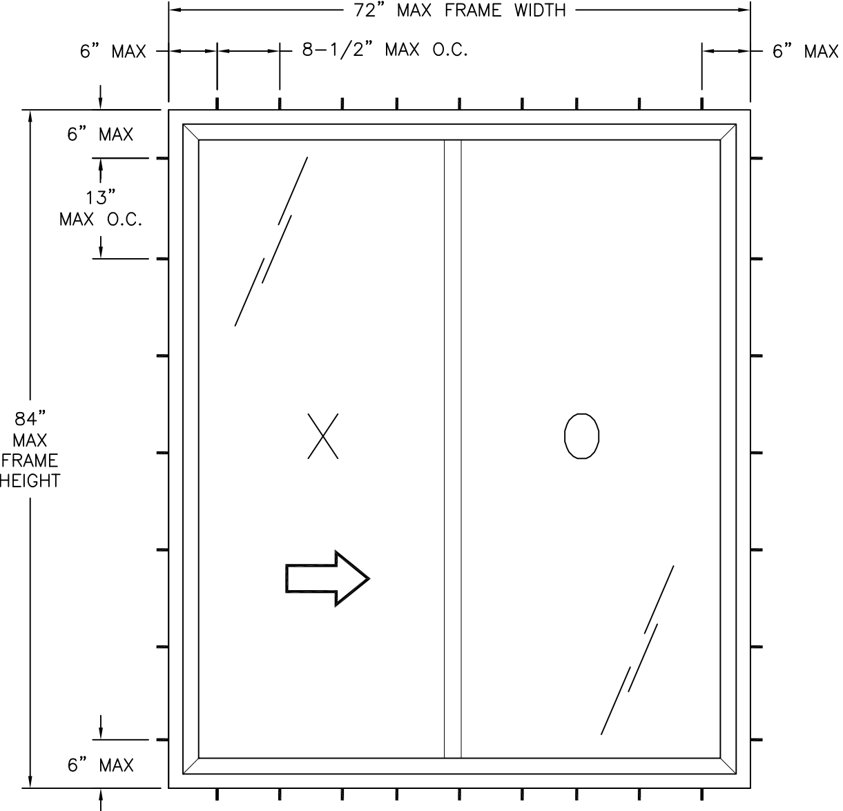
SERIES 176 SS VINYL HORIZONTAL SLIDING WINDOW EXTERIOR VIEW FRAME INSTALLATION
