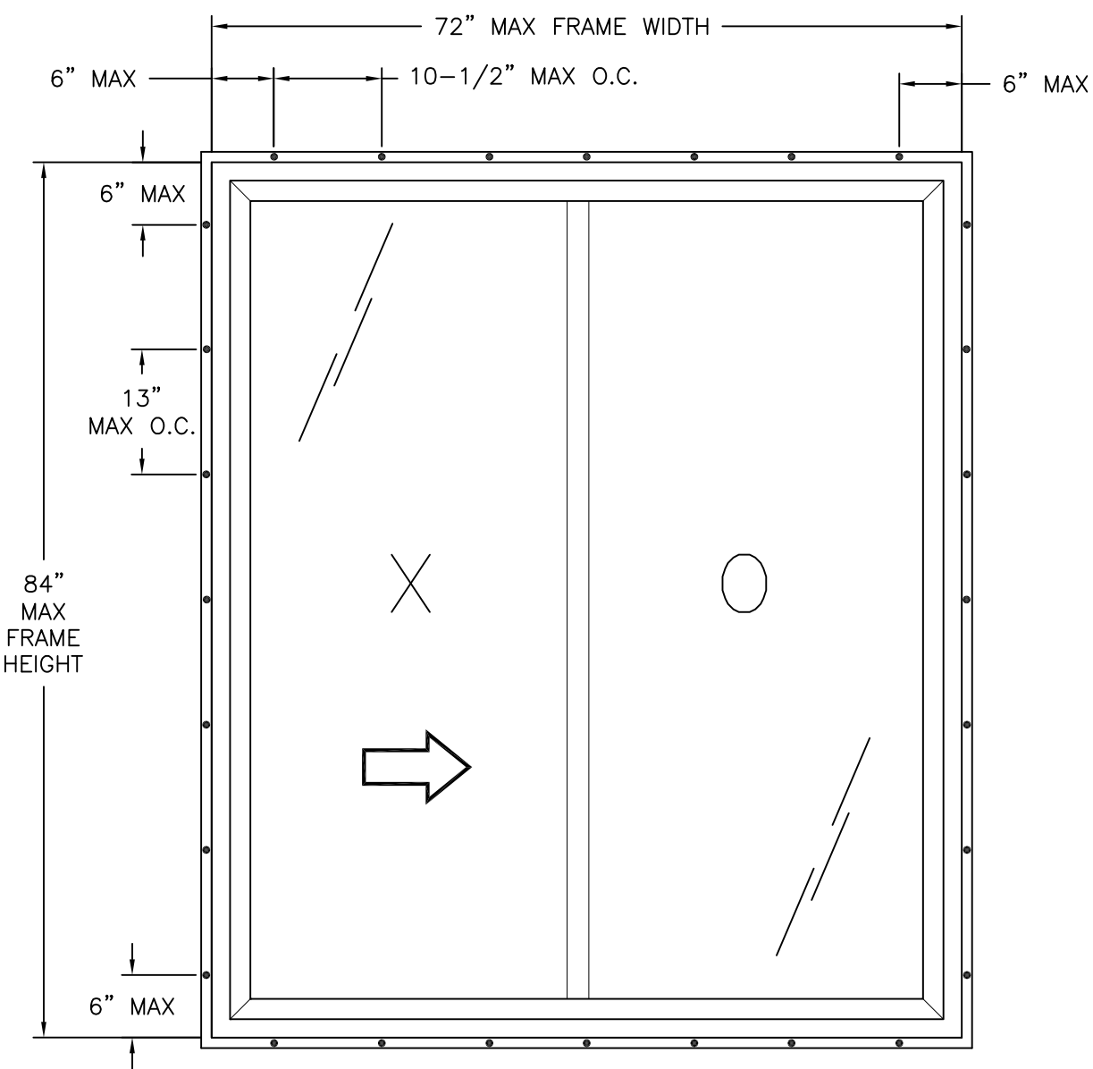
SERIES 176 SS VINYL HORIZONTAL SLIDING WINDOW EXTERIOR VIEW FIN INSTALLATION
