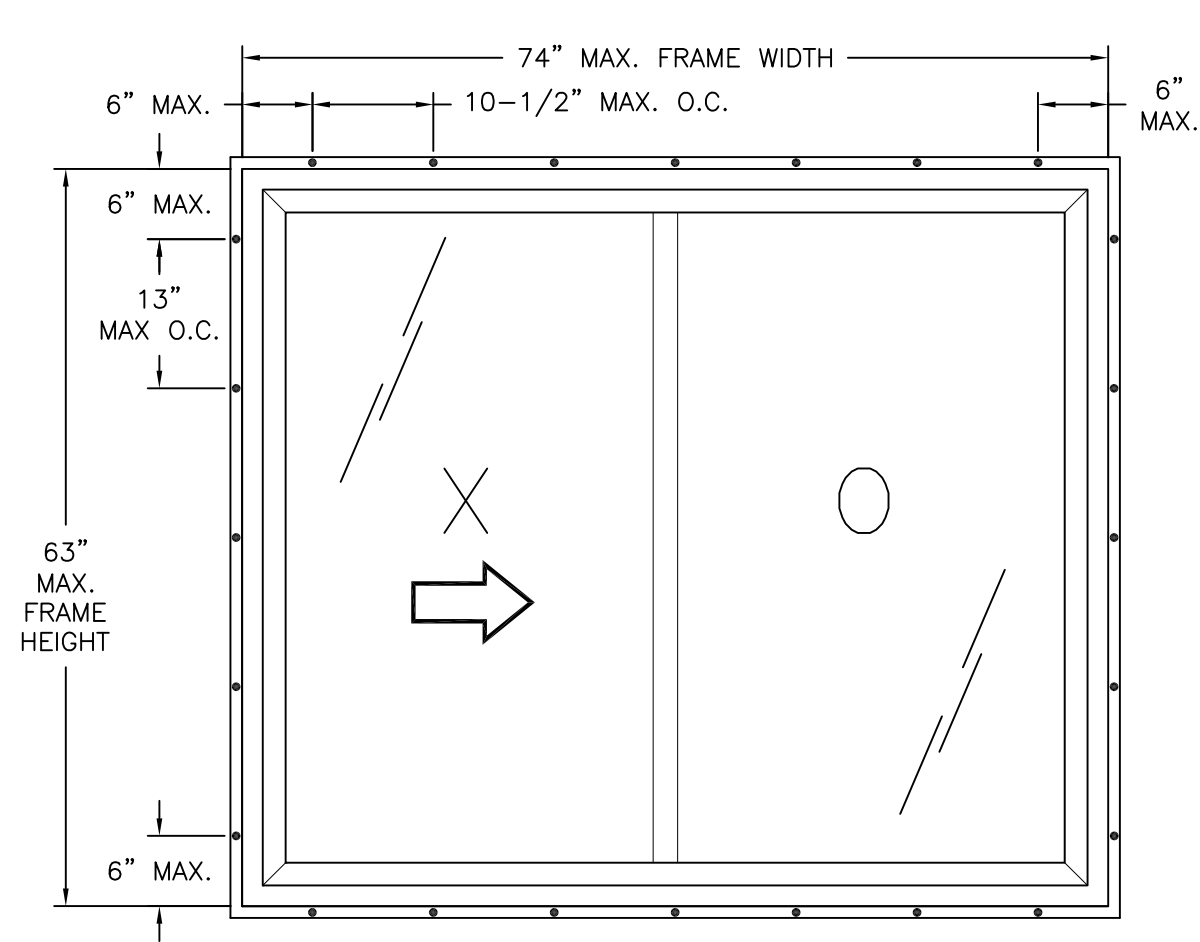
SERIES 176 SS VINYL HORIZONTAL SLIDING WINDOW EXTERIOR VIEW FIN INSTALLATION
