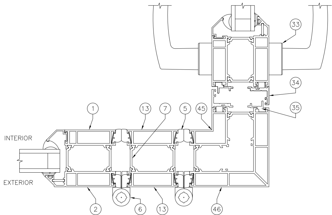
DETAIL H5. OPEN-OUT OUTSIDE 90-DEG. CORNER MULLION
