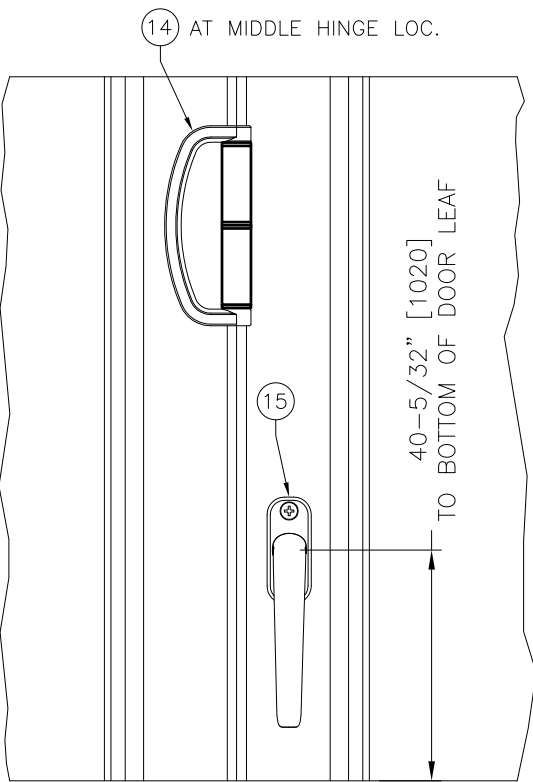
DETAIL D1. SECONDARY AND D-HANDLE (VIEW FROM INTERIOR)
