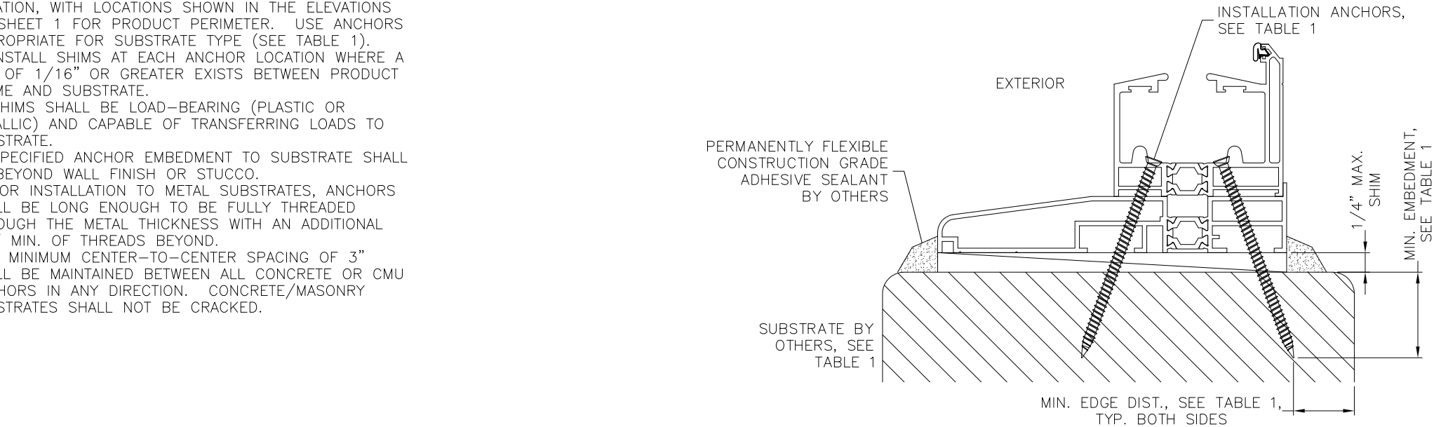
TYPICAL INSTALLATION STANDARD BOTTOM TRACK
