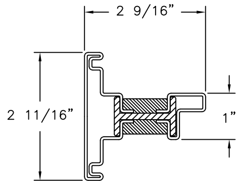
SASH RAIL AND STILE BRONZE (P1212)
