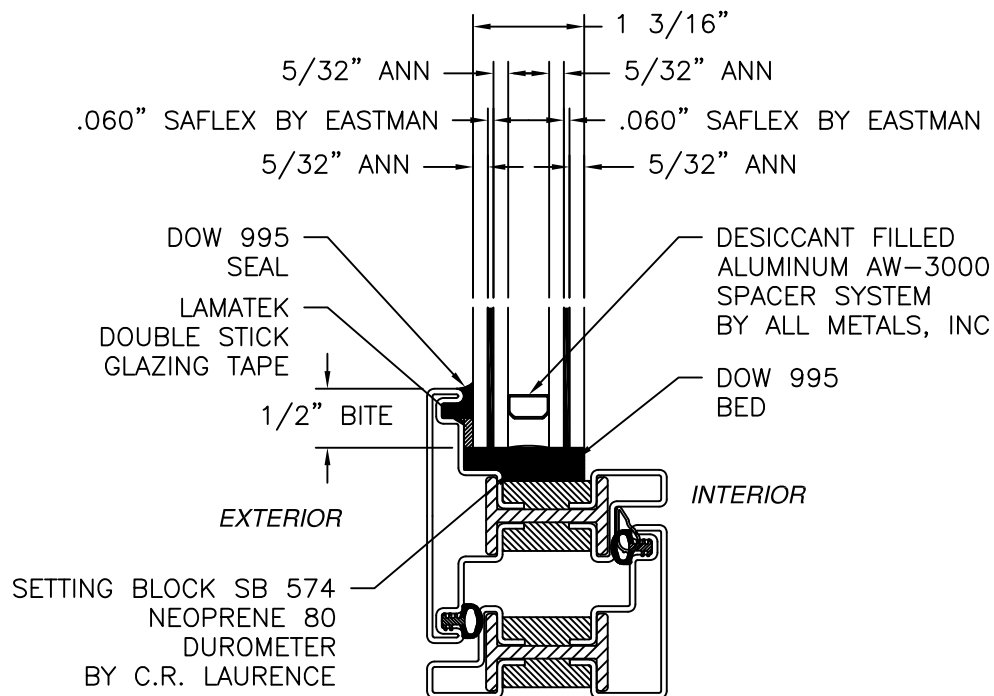
GLAZING DETAIL
