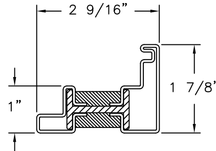
FRAME HEAD, SILL AND LEGS BRONZE (P1211)
