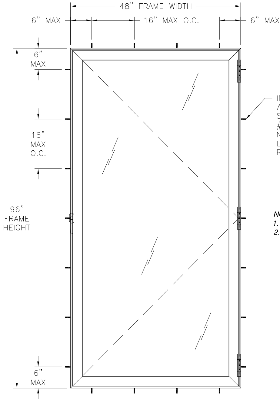
RWD40 C CASEMENT WINDOW EXTERIOR VIEW
