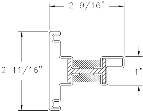
SASH RAIL AND STILE BRONZE (P1212)
