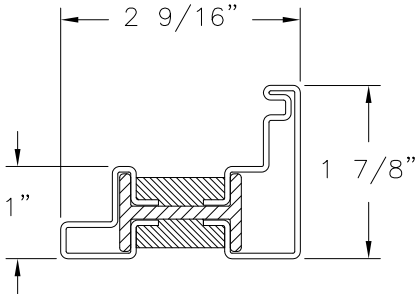
FRAME HEAD, SILL AND LEGS BRONZE (P1211)
