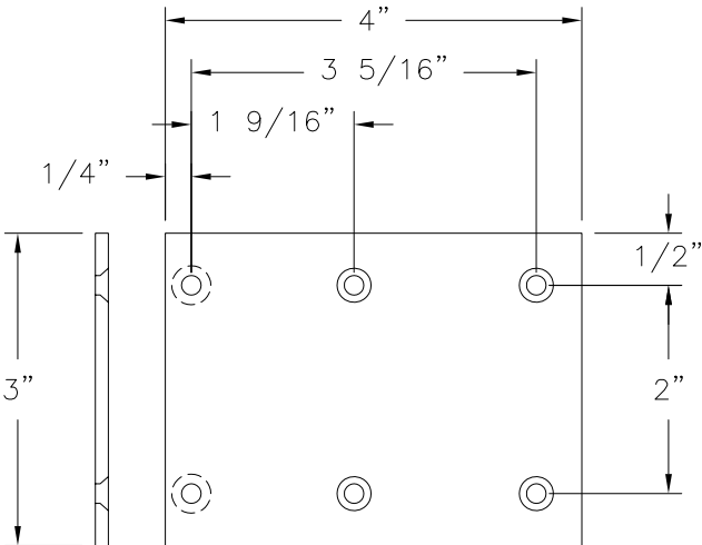
INSTALLATION BRACKET ALUMINUM 6063-T5 .125" THICK
