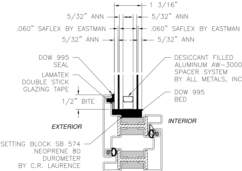
GLAZING DETAIL
