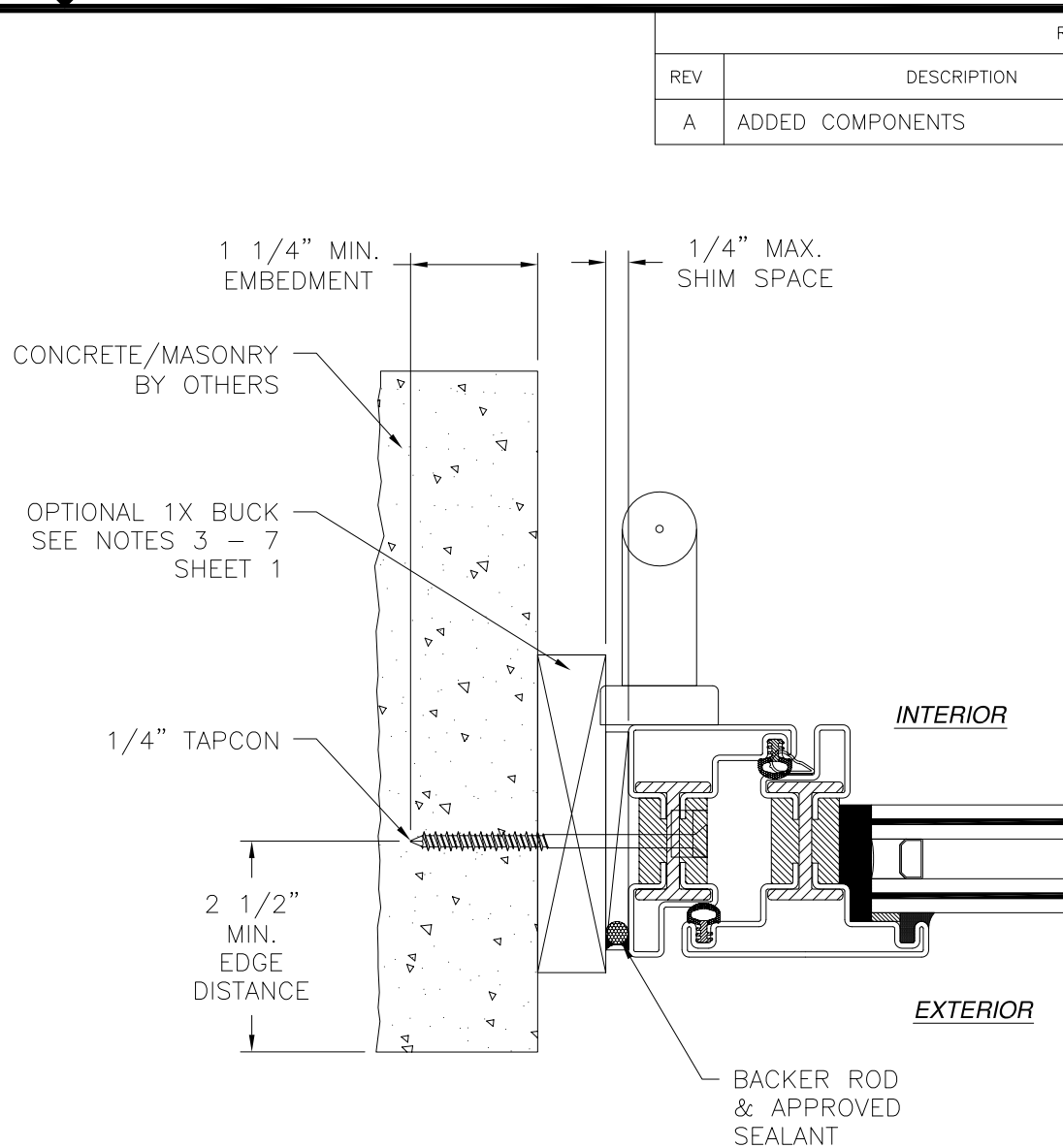
JAMB INSTALLATION DETAIL CONCRETE/MASONRY INSTALLATION
