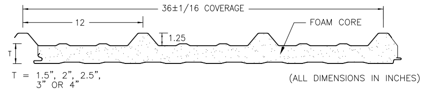
TOTALCLAD XRIB PANEL MIN 26 GA. EXT - INT PROFILES
