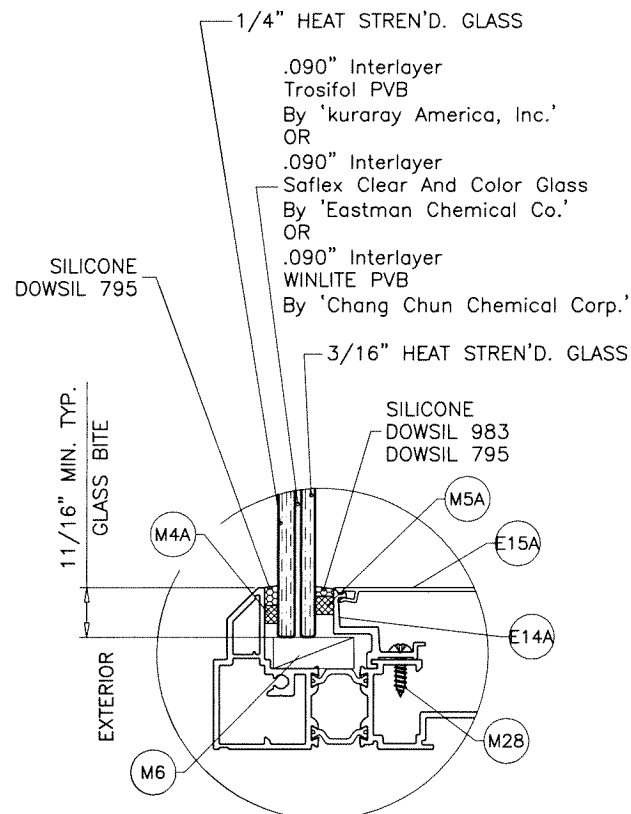
TRANSOM/SIDELITE
