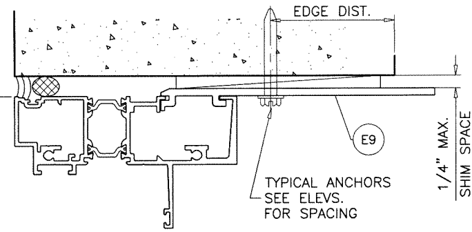
DOOR HEAD/JAMB
