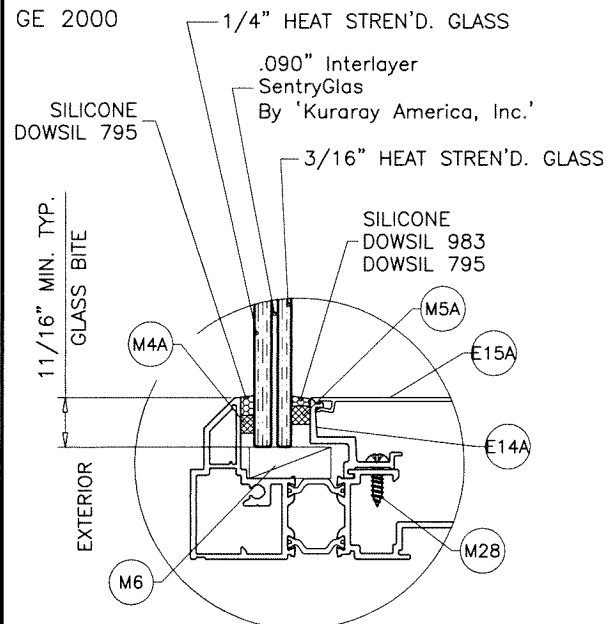
TRANSOM/SIDELITE
