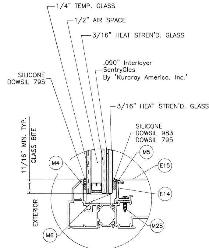
TRANSOM/SIDELITE
