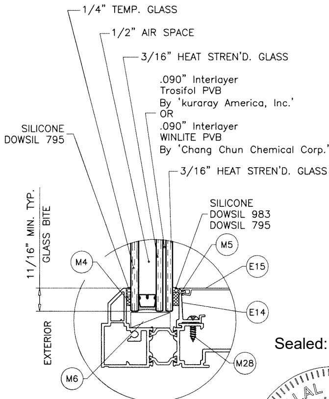
TRANSOM/SIDELITE
