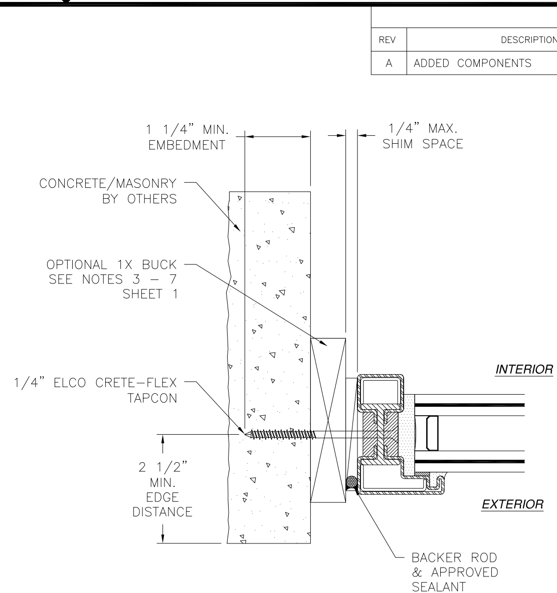
JAMB INSTALLATION DETAIL CONCRETE/MASONRY INSTALLATION
