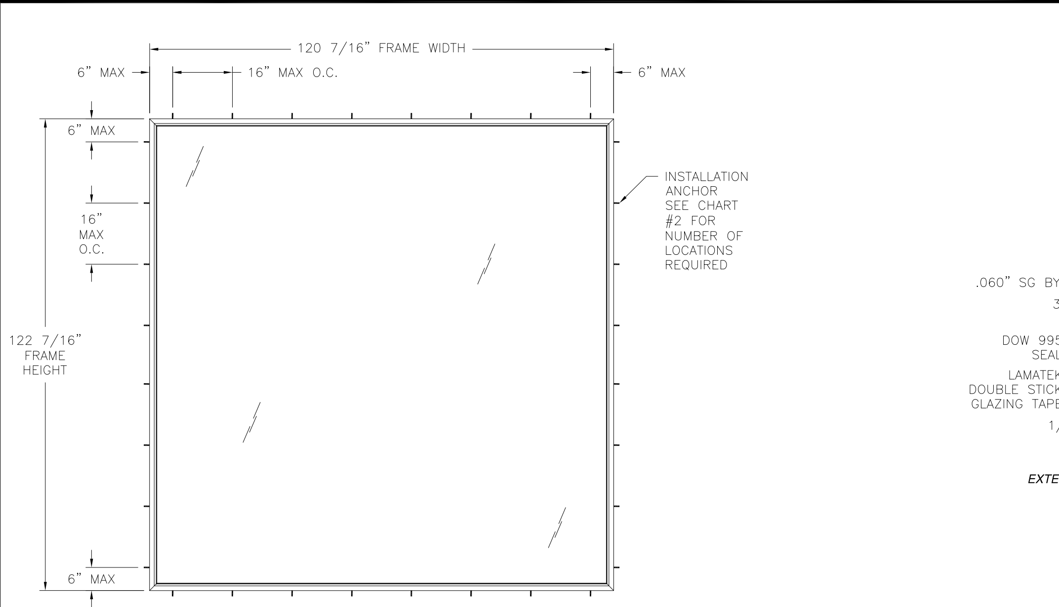
RWD40 B FIXED WINDOW EXTERIOR VIEW
