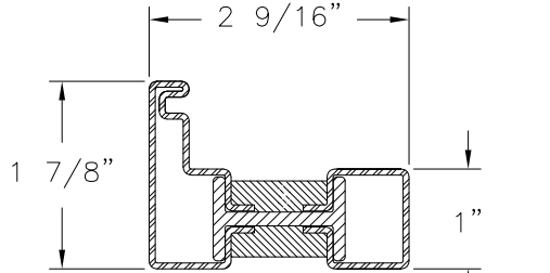
THERMALLY BROKEN BRONZE STILE/RAIL BRONZE .06 " THICK (1201)
