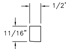
GLASS STOP (GSA) MAHOGANY .125" THICK
