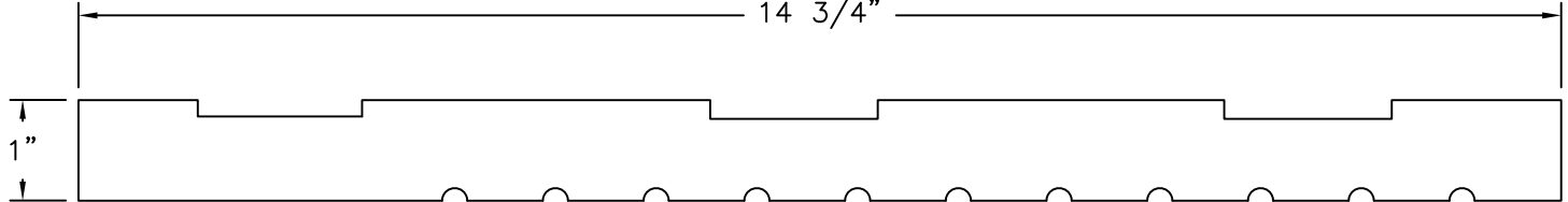
JAMB LEG - LEFT (J14.7A) MAHOGANY .125 " THICK
