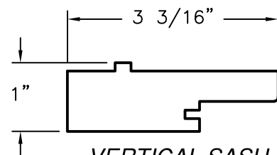
VERTICAL SASH STOP (SS3.1) MAHOGANY .125 " THICK
