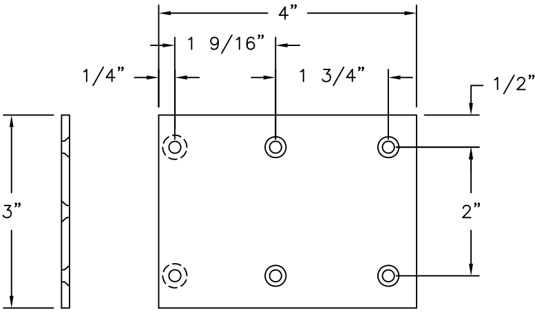
INSTALLATION BRACKET ALUMINUM 6063-T5 .125 " THICK
