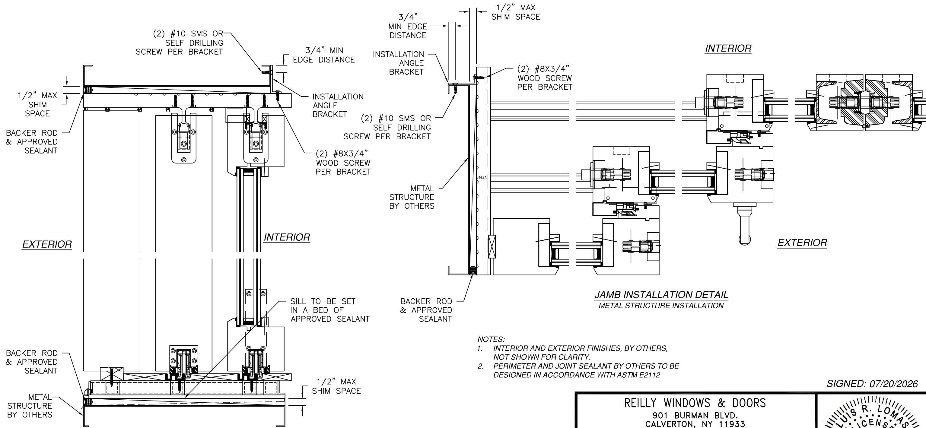
VERTICAL CROSS SECTION METAL STRUCTURE INSTALLATION
