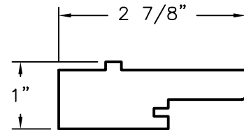
VERTICAL SASH STOP (SS2.8) MAHOGANY .125 " THICK
