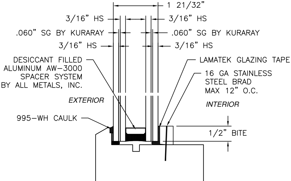
GLAZING DETAIL
