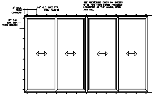
TYPICAL ELEVATION WITH FASTENER SPACING
