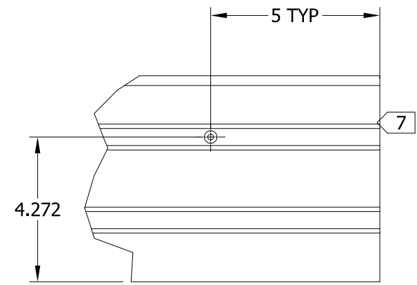
EXT ↓ DETAIL BA SCALE 1 / 4
