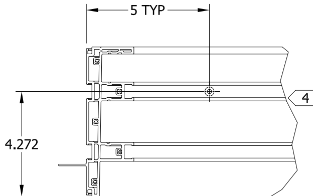
EXT ↓ DETAIL AN SCALE 1 / 4
