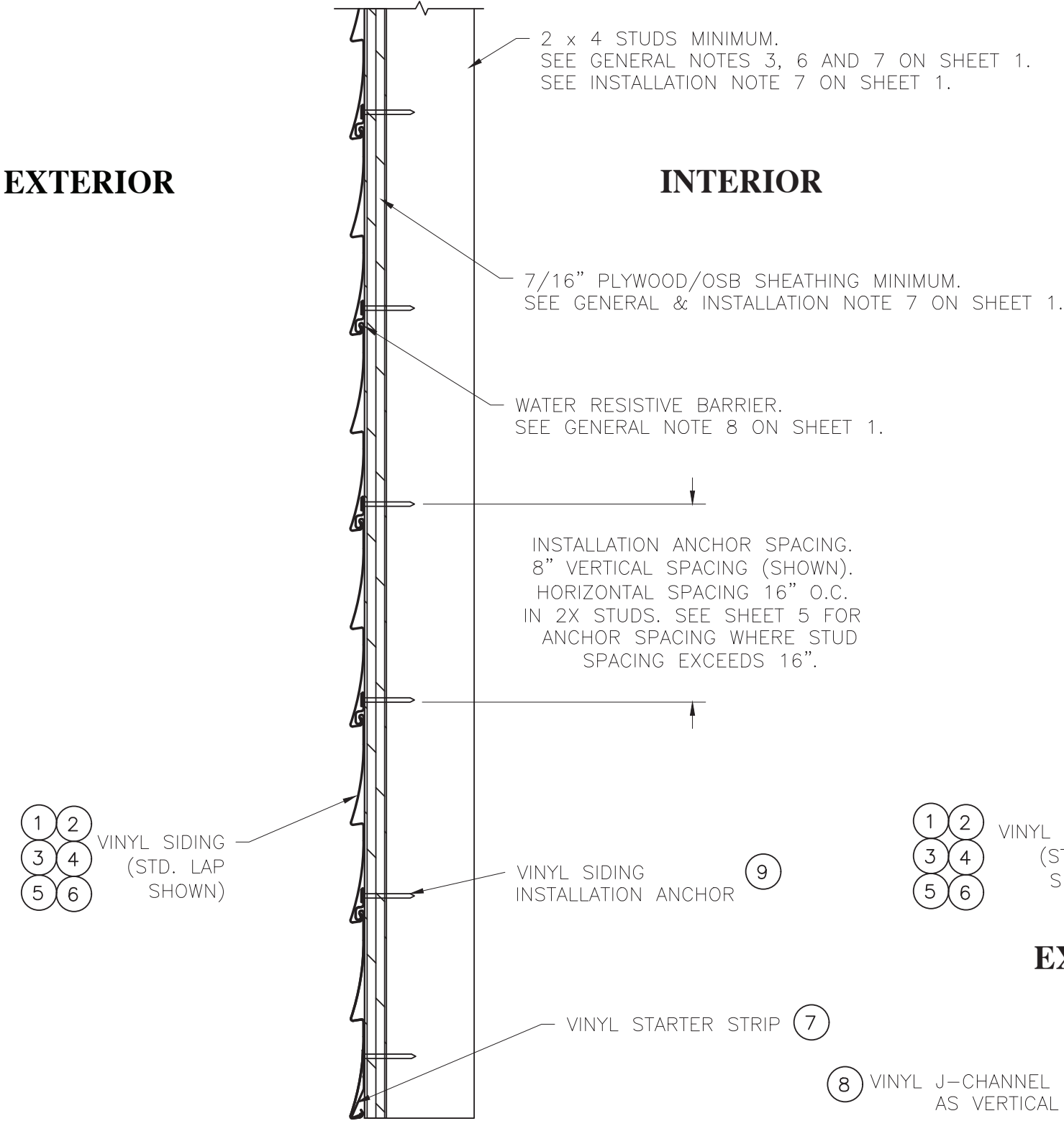
D4 INSTALLATION STARTER STRIP INSTALLATION
