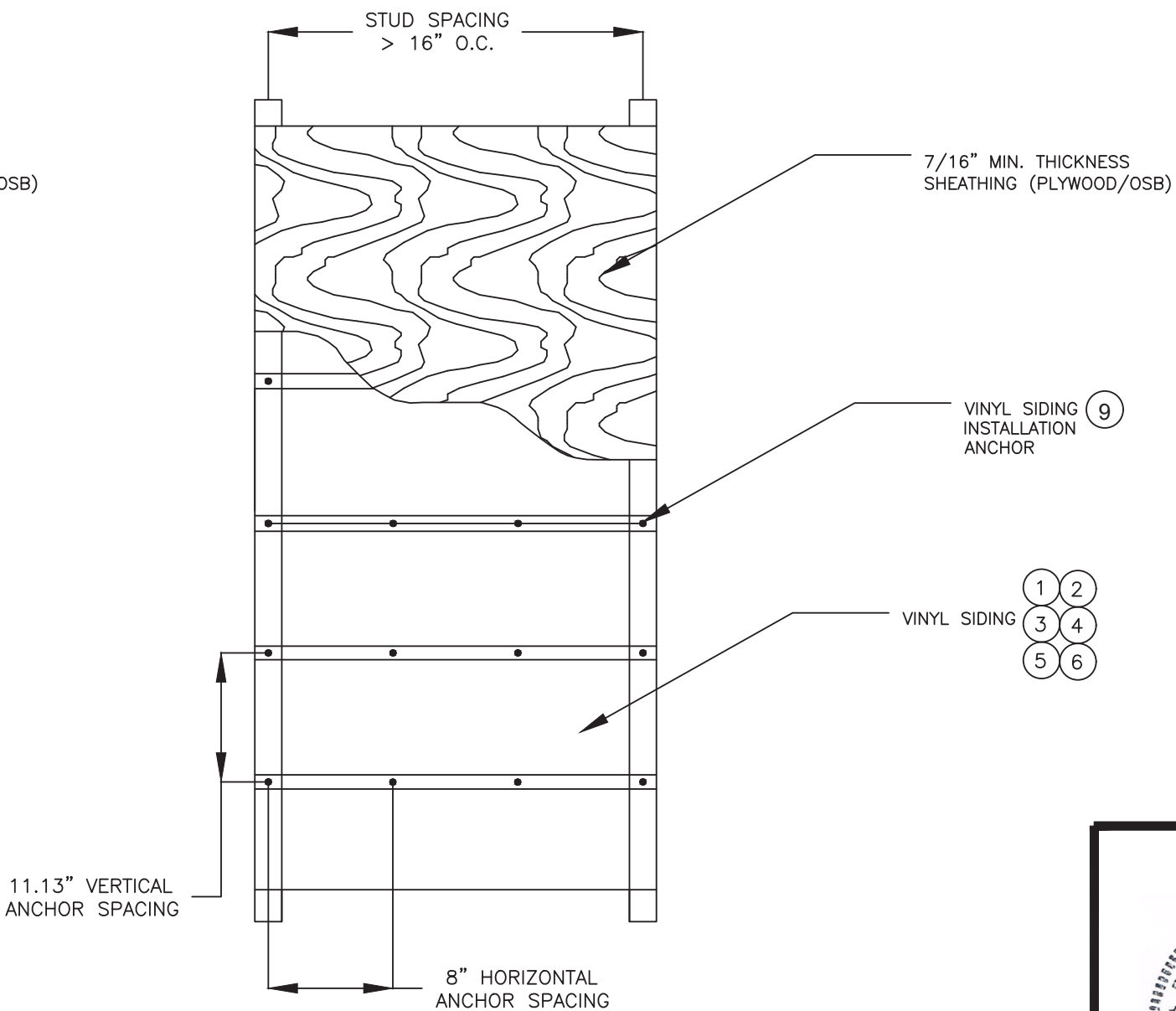
INSTALLATION ANCHORING FOR STUD SPACING EXCEEDING 16" MAXIMUM (24" O.C. SHOWN) (INSTALLATION ANCHOR EMBEDMENT INTO SHEATHING)
