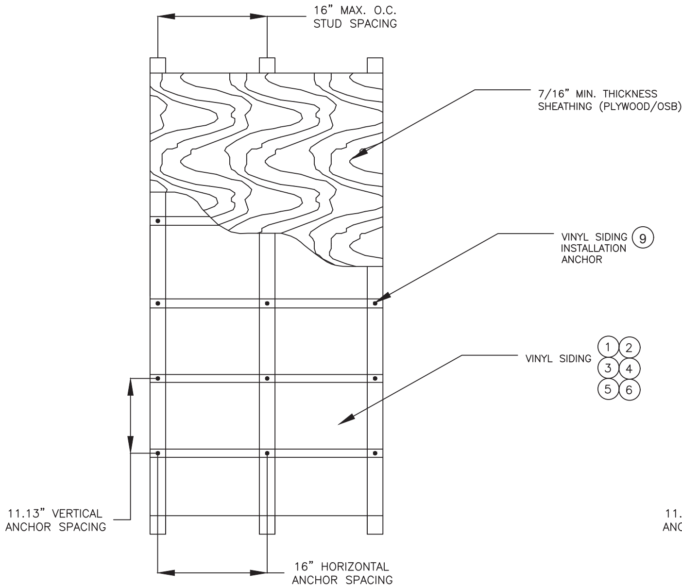
INSTALLATION ANCHORING FOR 16" MAXIMUM STUD SPACING (INSTALLATION ANCHOR EMMBEDMENT INTO 2X STUBS)
