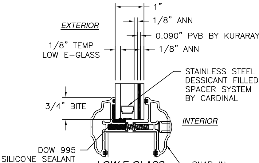
LOW E-GLASS GLAZING DETAIL
