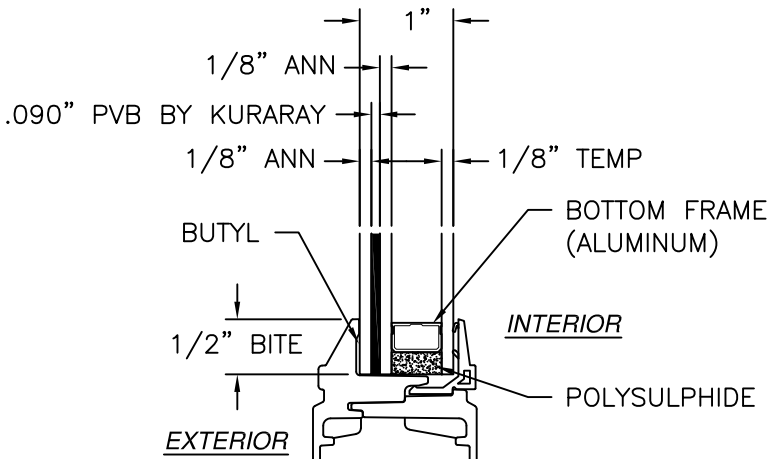
MINI-BLIND GLAZING DETAIL
