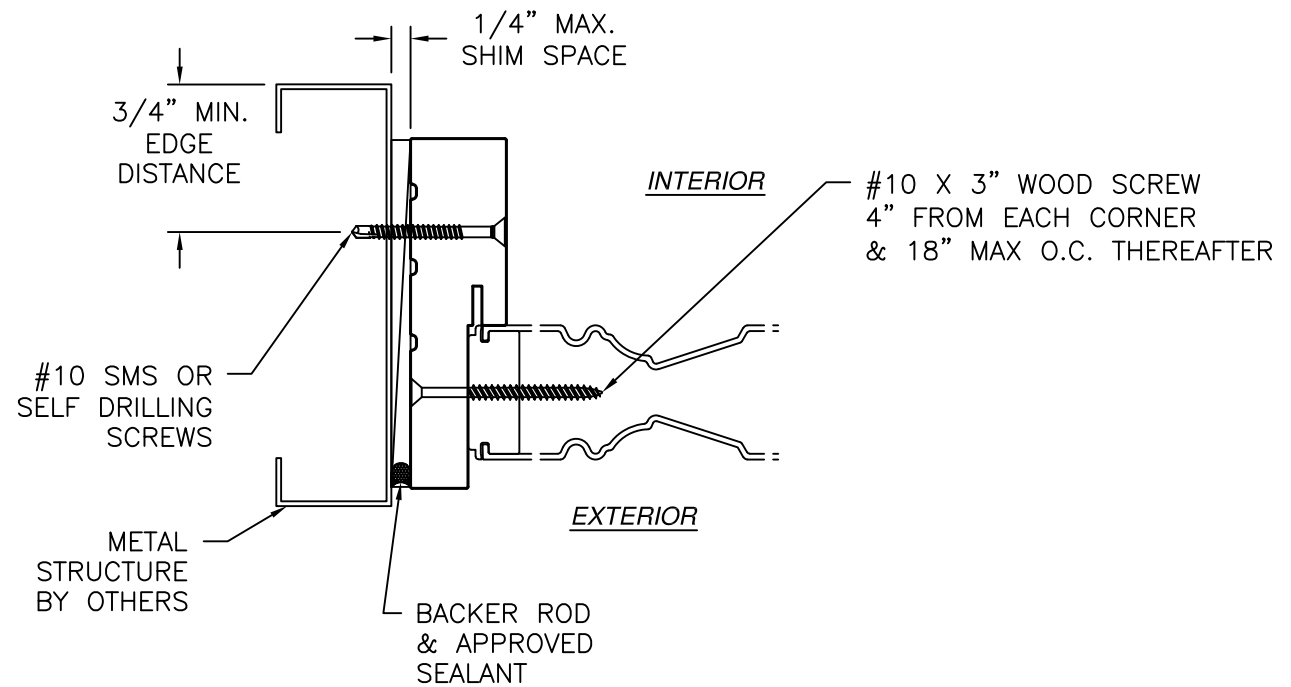
JAMB INSTALLATION DETAIL METAL STRUCTURE INSTALLATION
