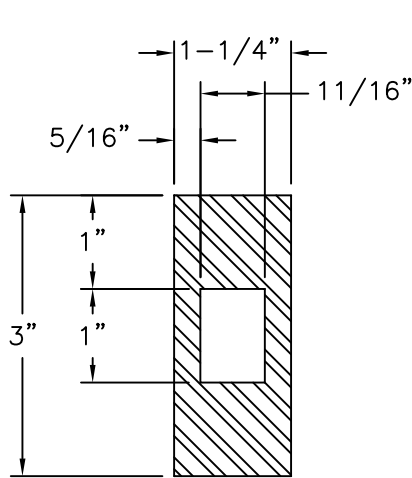
1 1/4\"X3\" TUBE MULLION ALUMINUM 6063-T6 .125\" THICK EFFECTIVE MOMENT OF INERTIA: 3.050 IN^4 EFFECTIVE SECTION MODULUS: 1.008 IN^3
