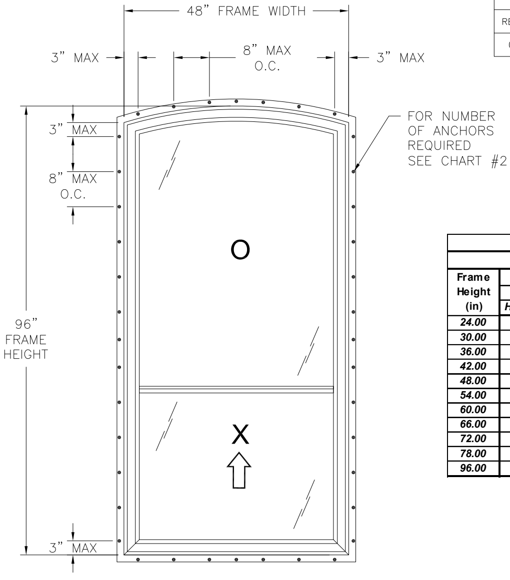
1620/1621 SH REINFORCED DESIGNER EXTERIOR VIEW FIN INSTALLATION
