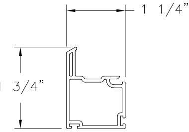
BOTTOM SASH/STILE EXTRUDED PVC (V-670)
