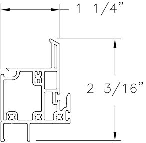
MEETING RAIL EXTRUDED PVC (V-1016)
