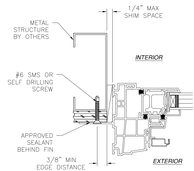
JAMB INSTALLATION DETAIL METAL STRUCTURE INSTALLATION
