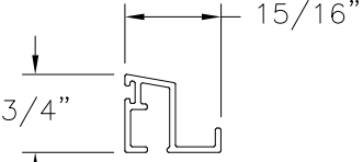
OPERABLE SCREEN TRACK W/O LEG ALUMINUM 6063-T5 (M-2341)
