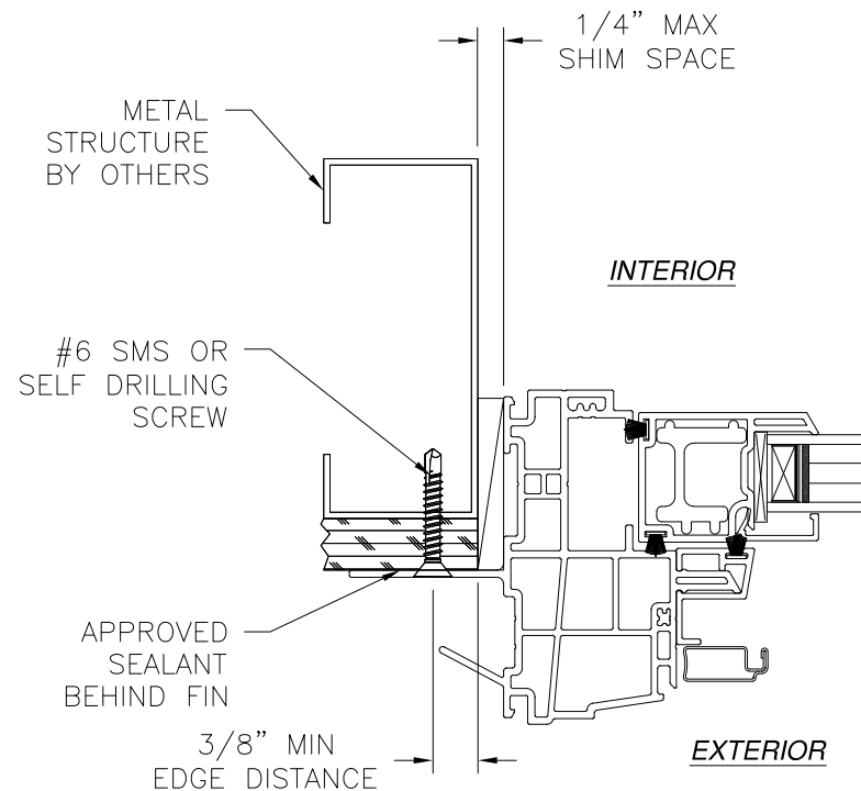
JAMB INSTALLATION DETAIL METAL STRUCTURE INSTALLATION
