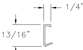
GLAZING BEAD RIGID PVC (V-904)
