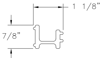
STILES REINFORCEMENT ALUMINUM 6063-T5 (M-2266)
