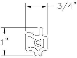
MEETING RAIL REINFORCEMENT ALUMINUM 6063-T5 (AE-000162)
