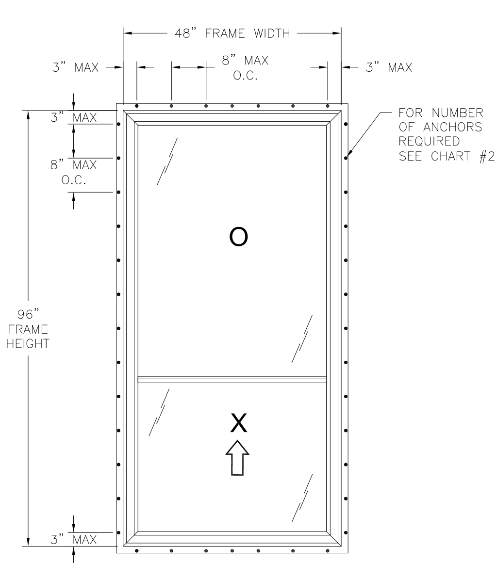
1620/1621 SH REINFORCED RECTANGULAR EXTERIOR VIEW FIN INSTALLATION
