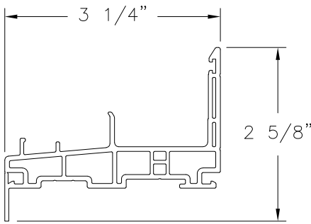
SILL WITH FLANGE EXTRUDED PVC (V-1015)
